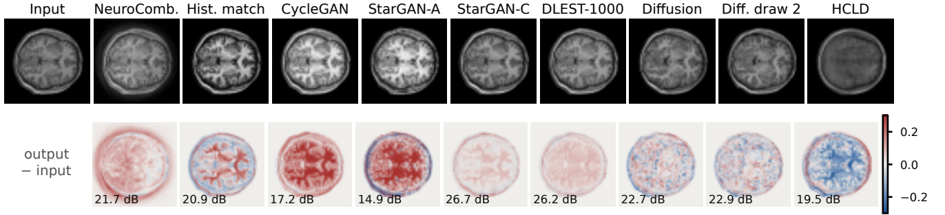
Fig. 2. One source test subject (chosen as the median of PSNR averaged over outputs). Bottom: output minus input, with PSNR. HCLD loses anatomical detail; diffusion adds texture that differs between draws.
