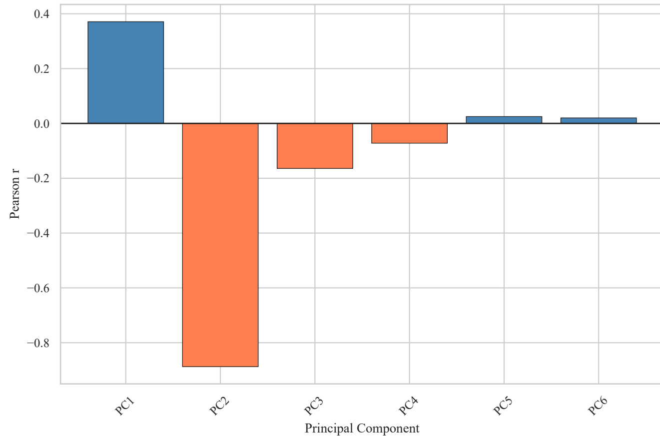
PC Correlation with LPI Target
