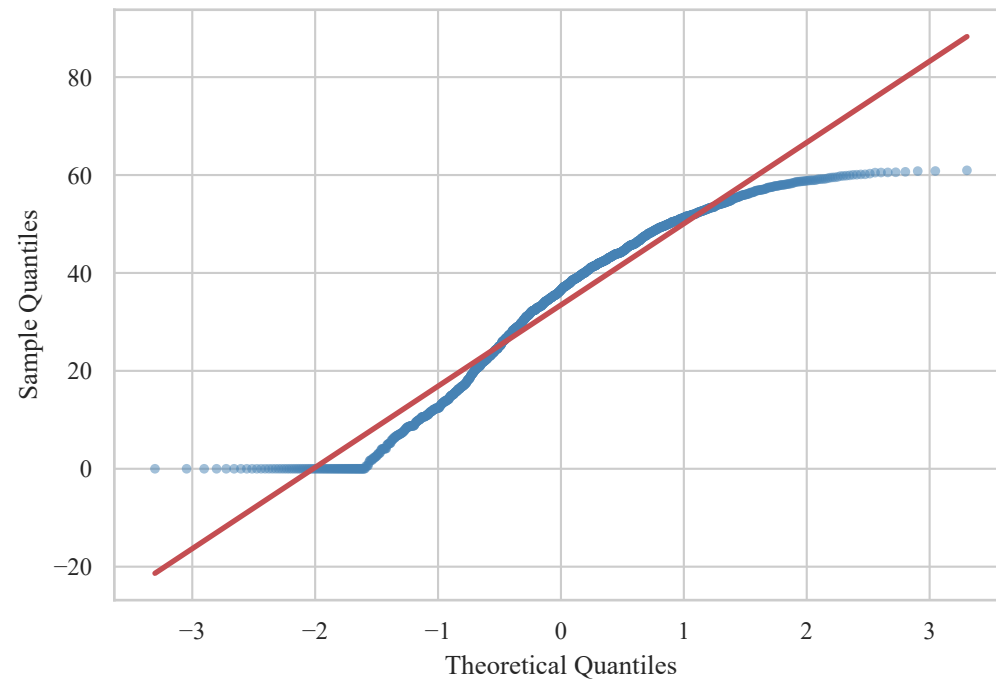
Q-Q Plot of LPI
