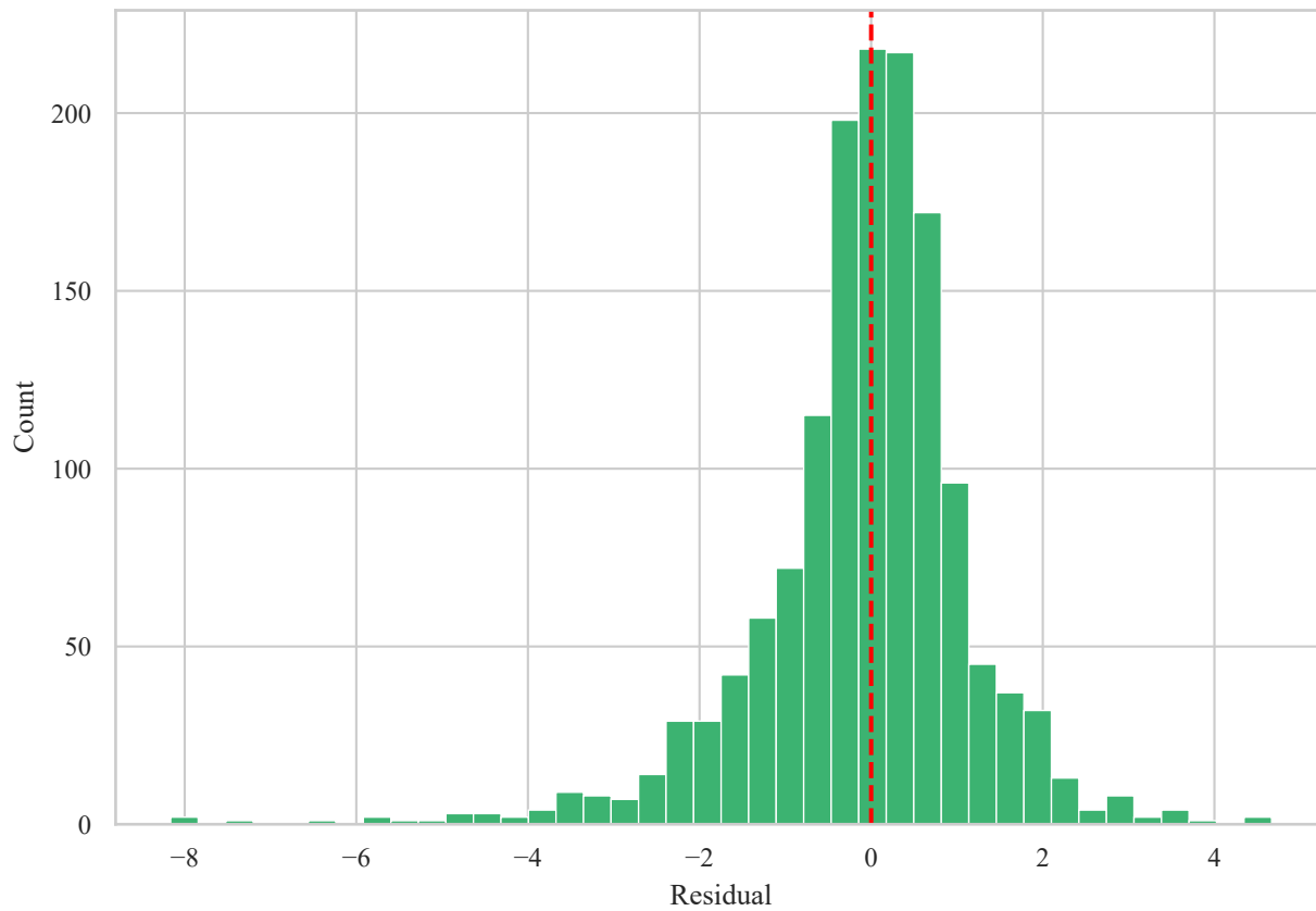
Residual Distribution
