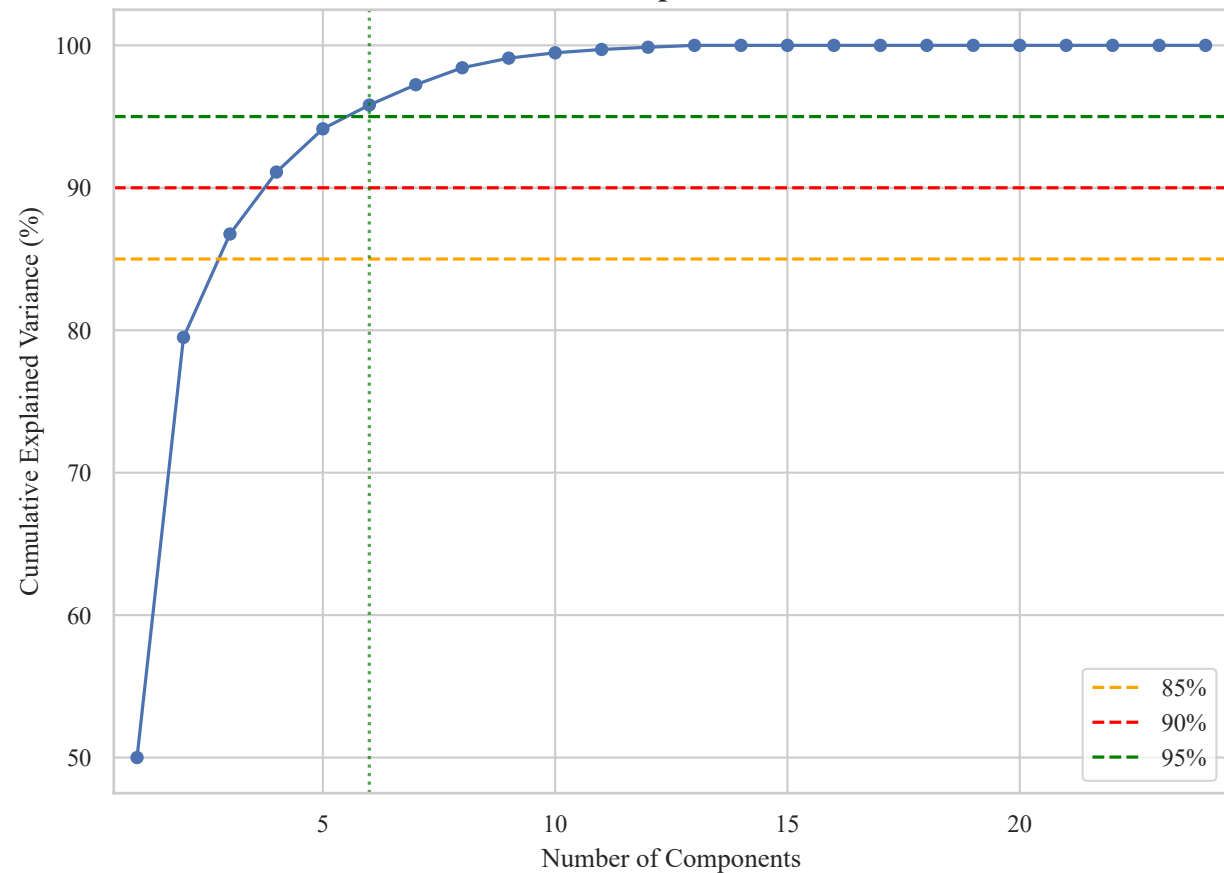
Cumulative Explained Variance
