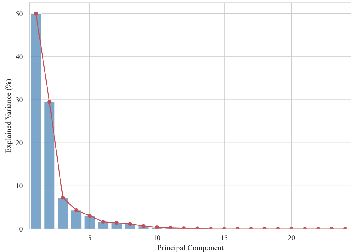
Scree Plot
