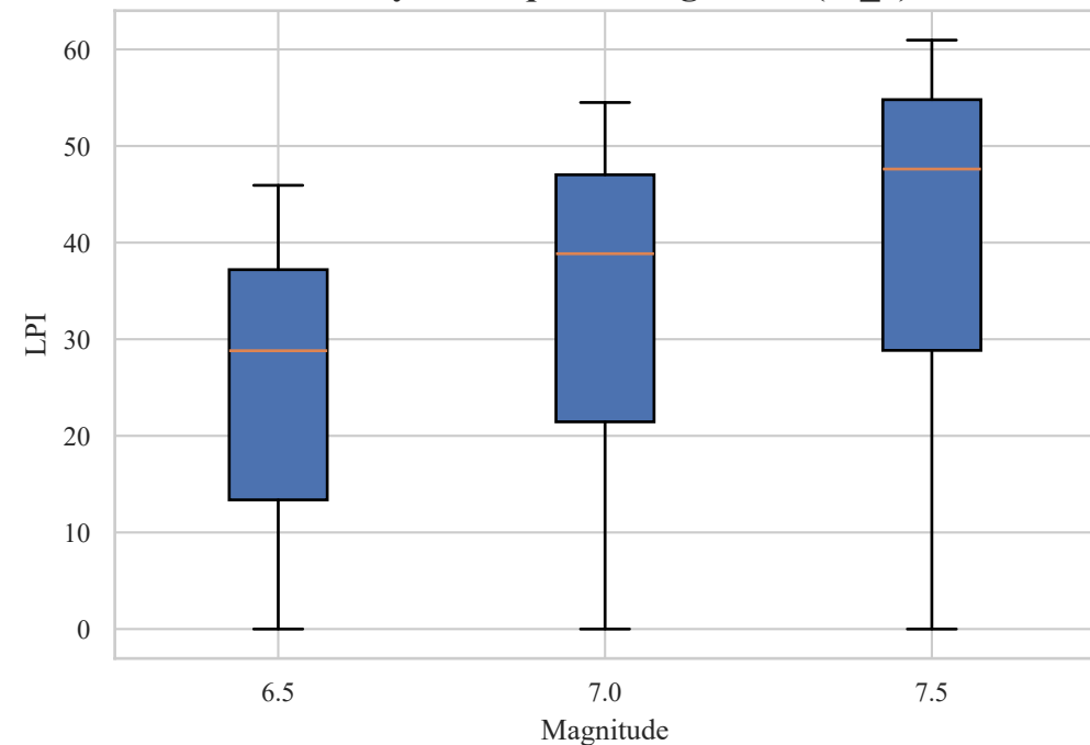
LPI by Earthquake Magnitude (M_3)
