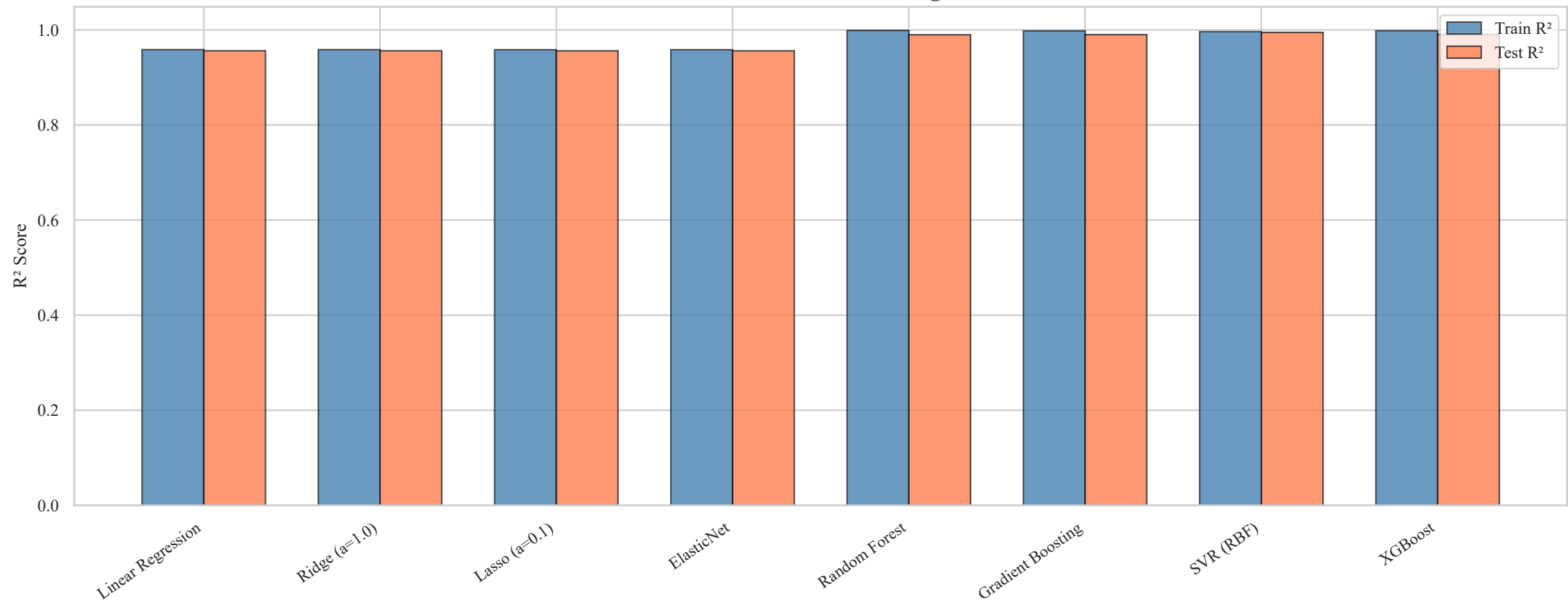
Train vs Test R^2 — Overfitting Check
