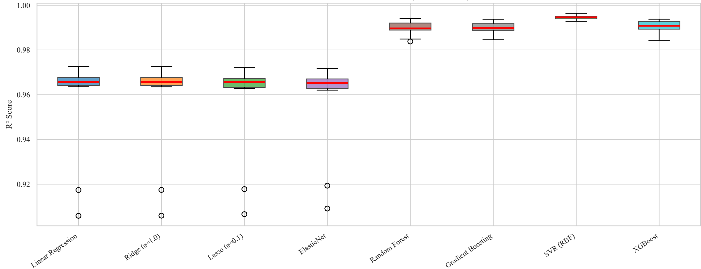
Per-Fold R^2 Score Distribution (10-Fold CV)
