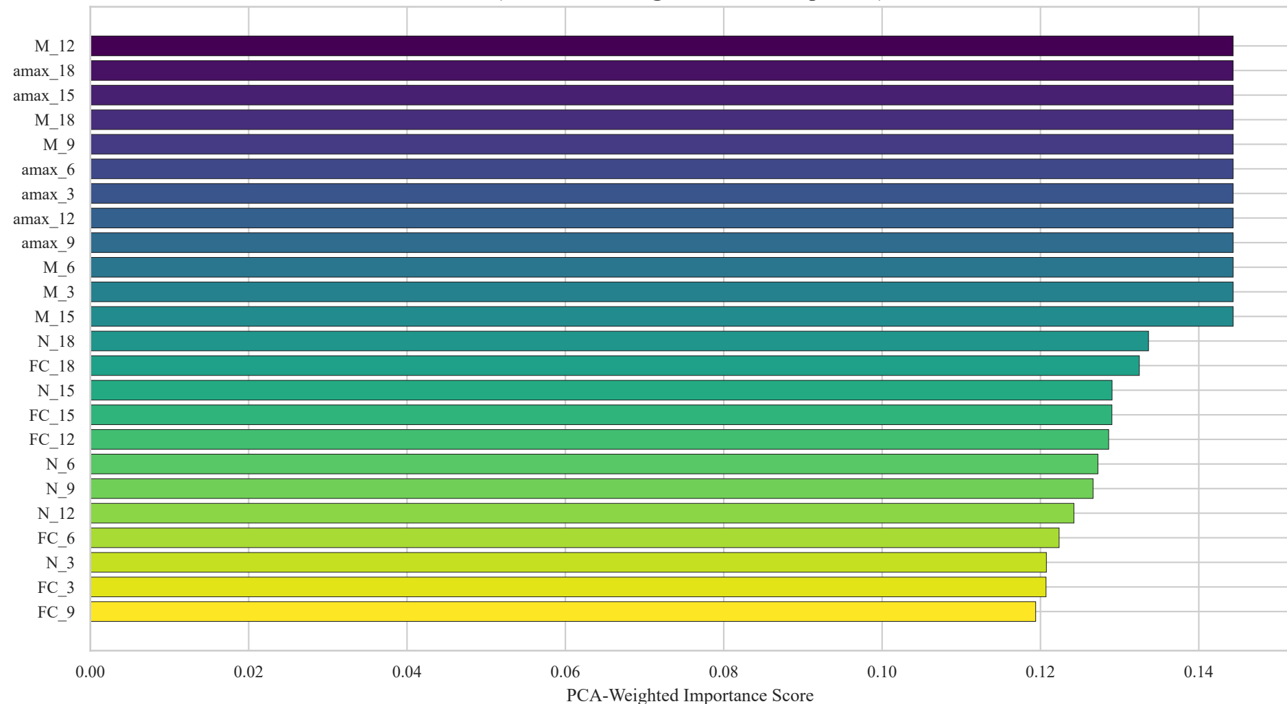
Original Feature Importance (via PCA Loadings \times Variance Explained)
