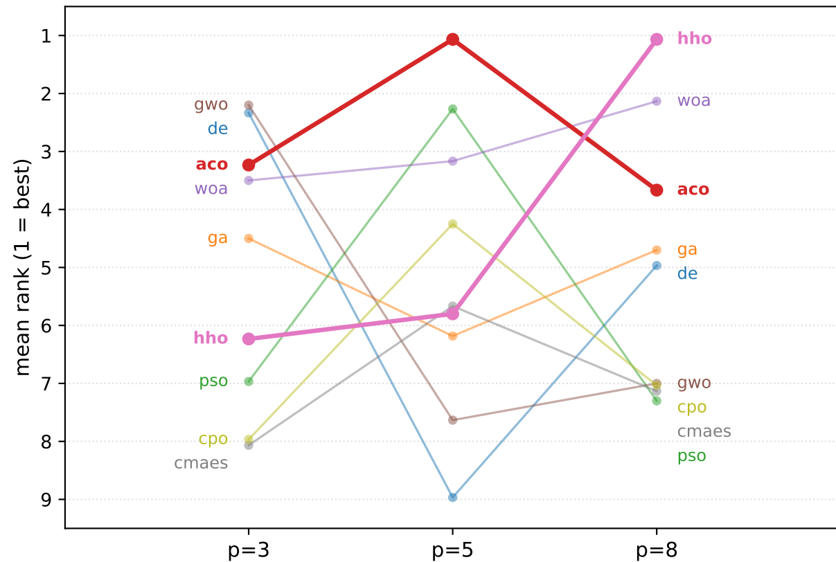
Operator ranking vs QAOA depth (crossing lines = ranking does not transfer)
