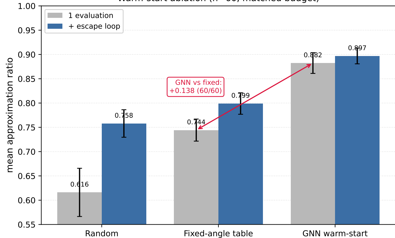
Warm-start ablation (n=60, matched budget)
