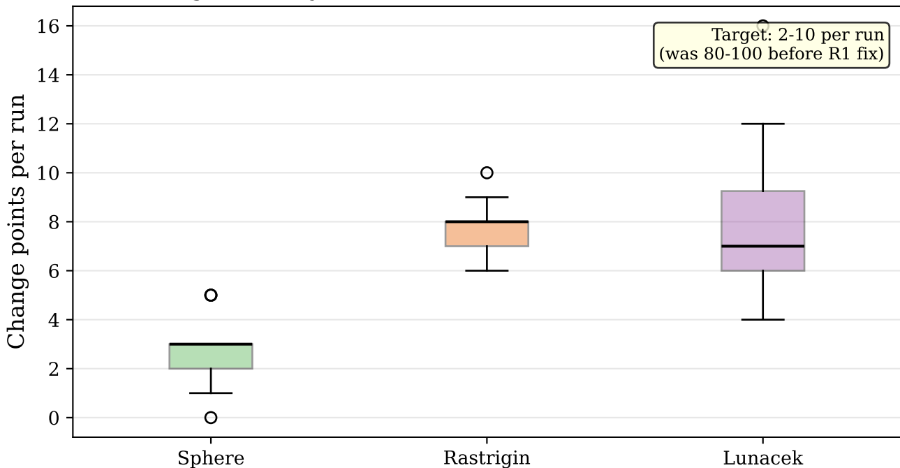
Page-Hinkley Detections (20 seeds, D=10, 5000 FEs)
