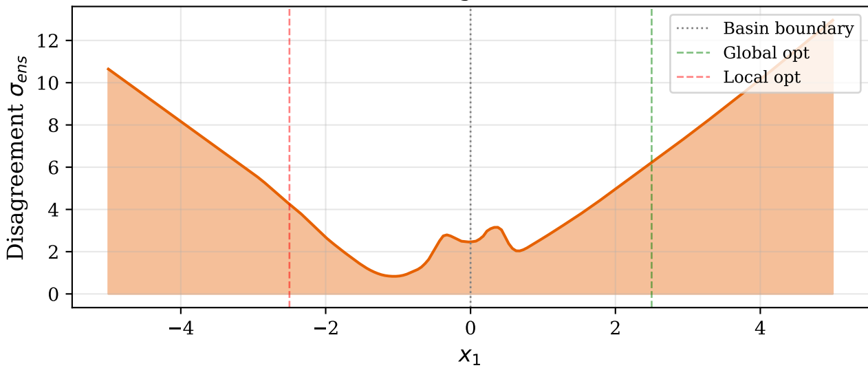
Ensemble Disagreement Profile
