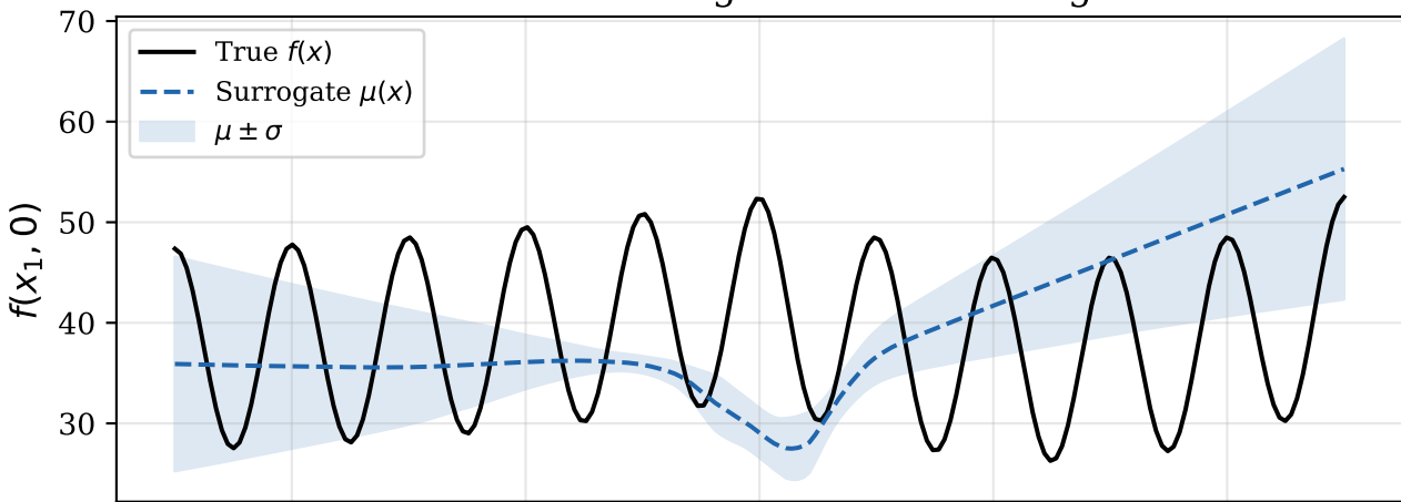
Lunacek bi-Rastrigin: True vs Surrogate
