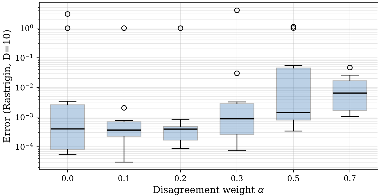
Sensitivity of \alpha (10 seeds, 5000 FEs)
