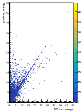
electron
