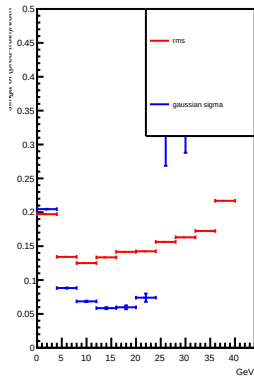
photon
