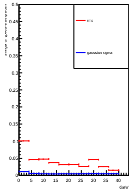
pion
