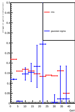
electron
