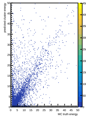
neutron
