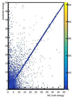
pion
