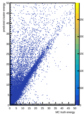
photon
