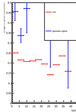
neutron
