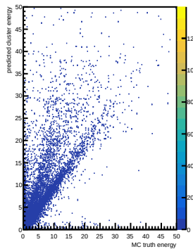
photon cluster energy
