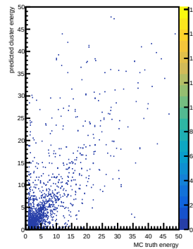
neutron cluster energy
