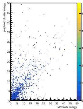
K0 cluster energy
