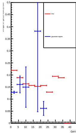
electron
