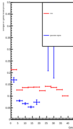
photon
