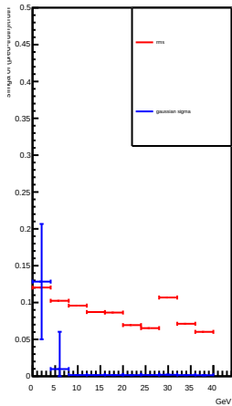
pion
