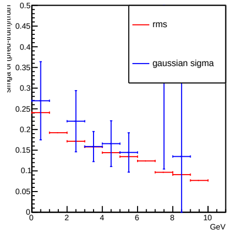
photon
