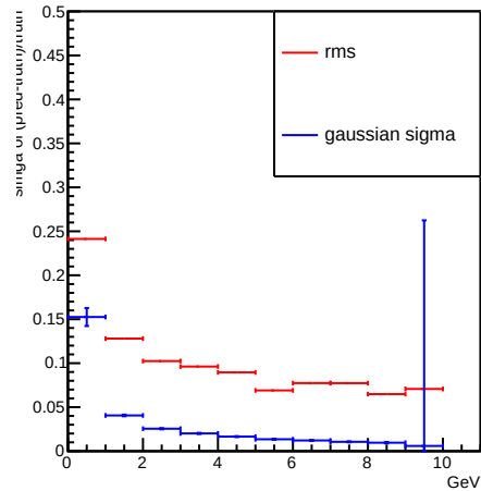
electron
