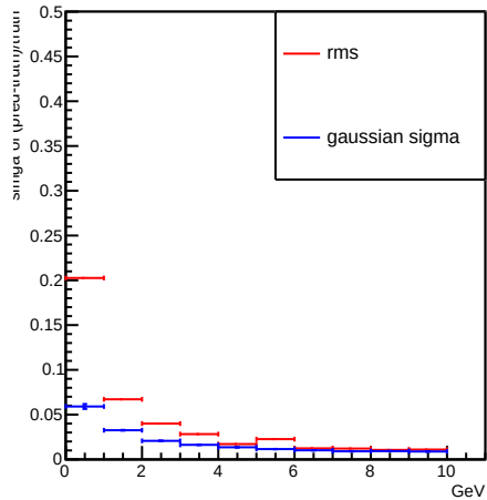
pion
