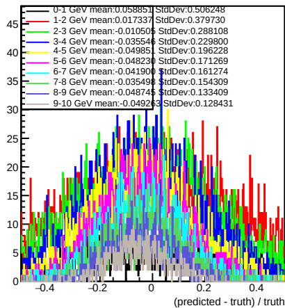
pion
