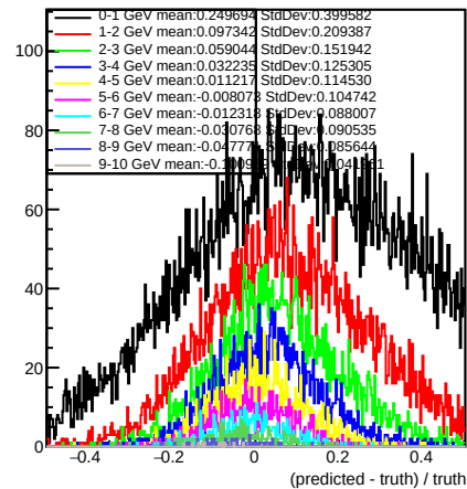
photon
