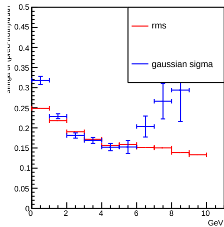
electron
