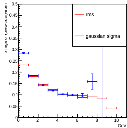
photon
