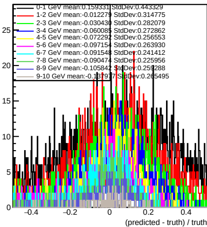
electron
