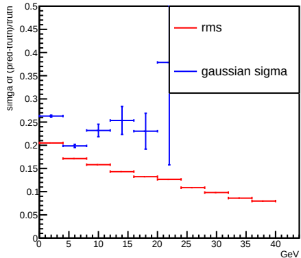
pion
