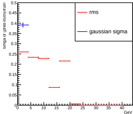
electron
