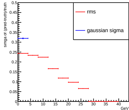
photon
