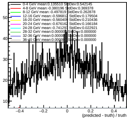
electron
