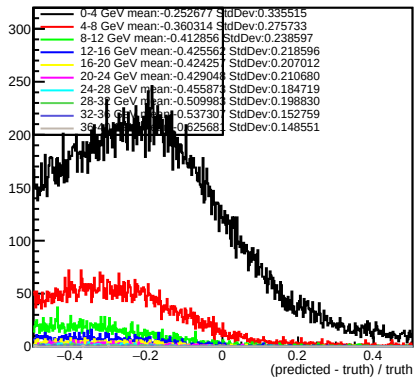
pion
