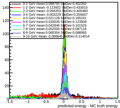
pion
