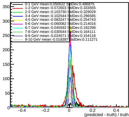
pion
