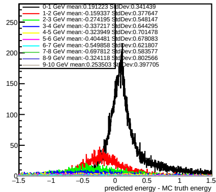
photon
