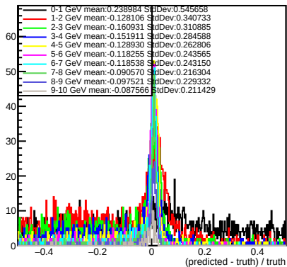
electron
