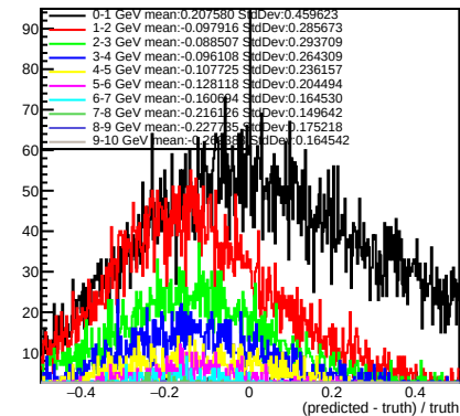
photon
