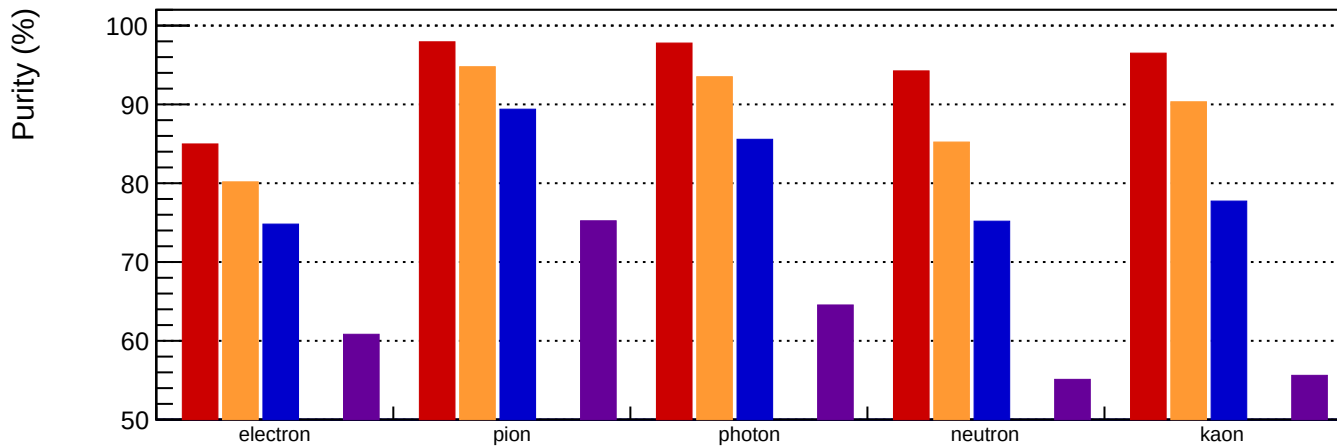
Purity
