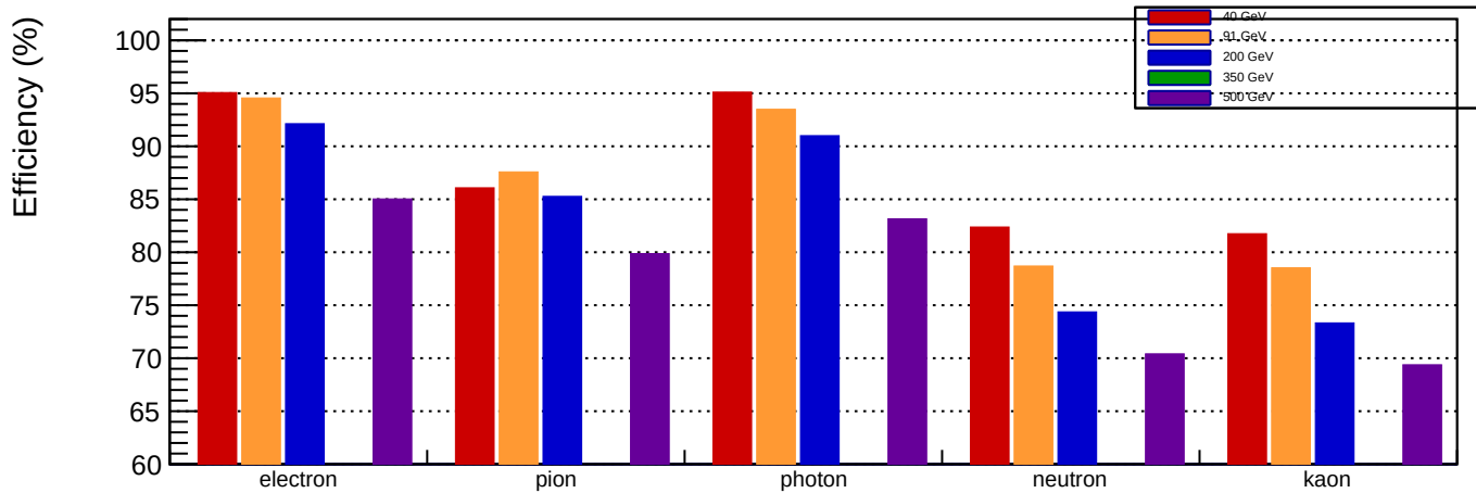
Efficiency
