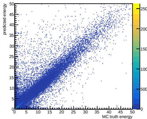
pion cluster energy
