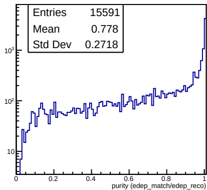
electron purity (MC energy&gt;1 GeV)
