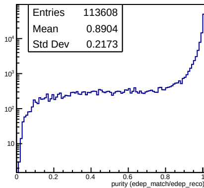
photon purity (MC energy&gt;1 GeV)
