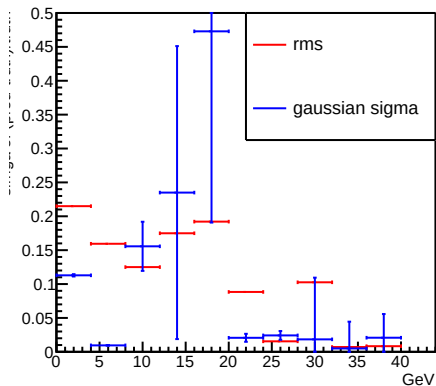
electron
