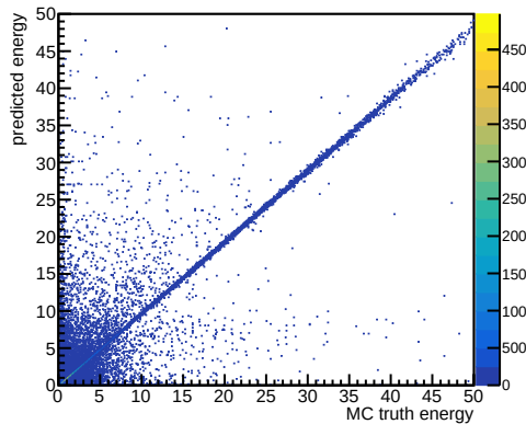
pion
