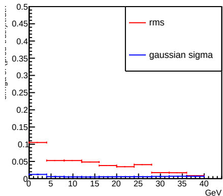
pion
