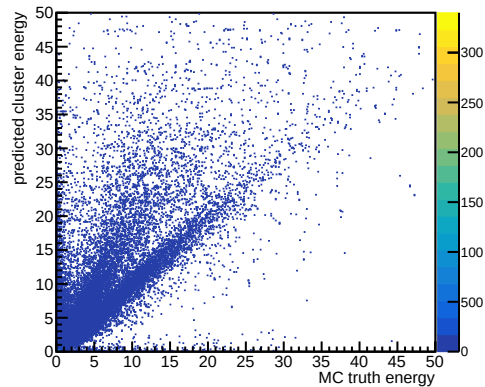
photon
