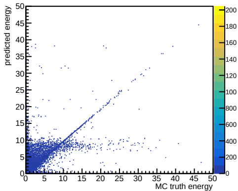
electron
