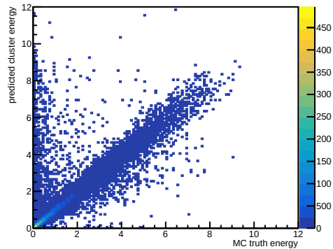
photon cluster energy
