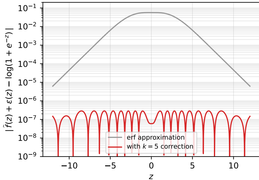
error across z ( k = 5 )
