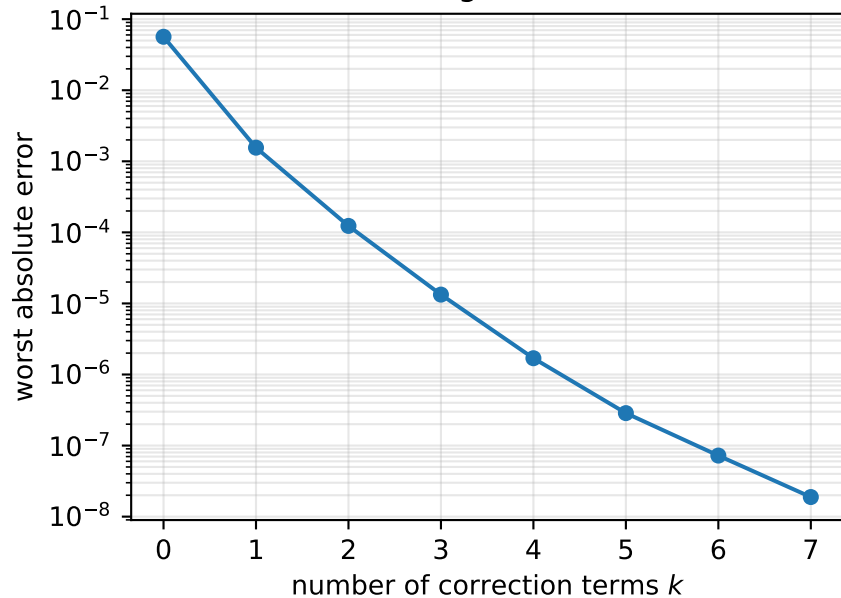
convergence in k
