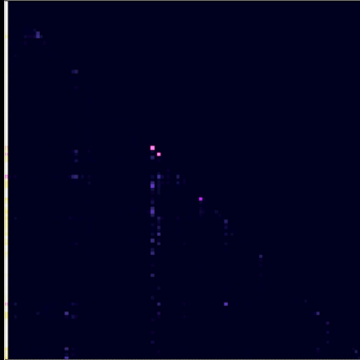
Sparse-GPT
