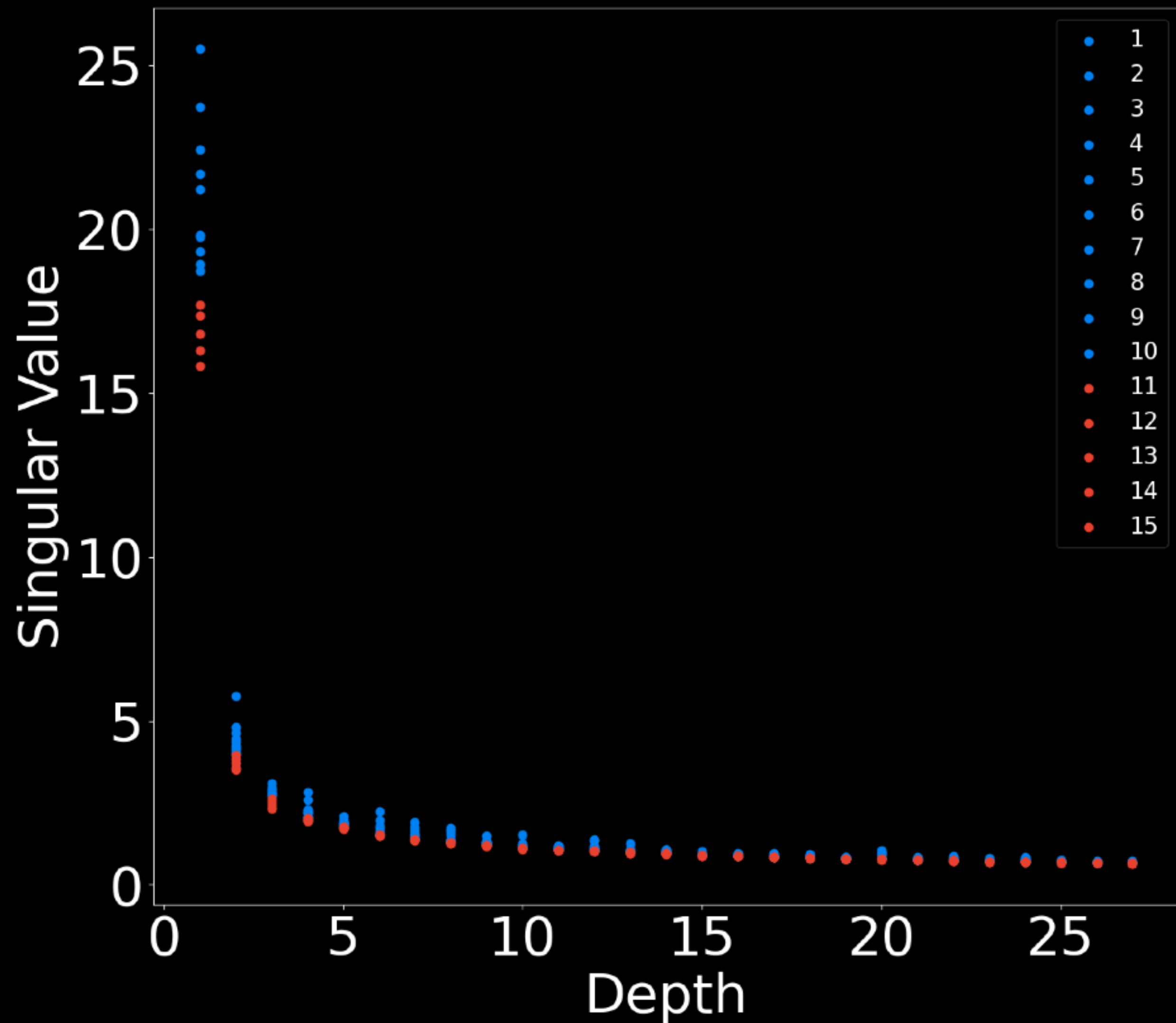
Gemma-7b (Untrained)
