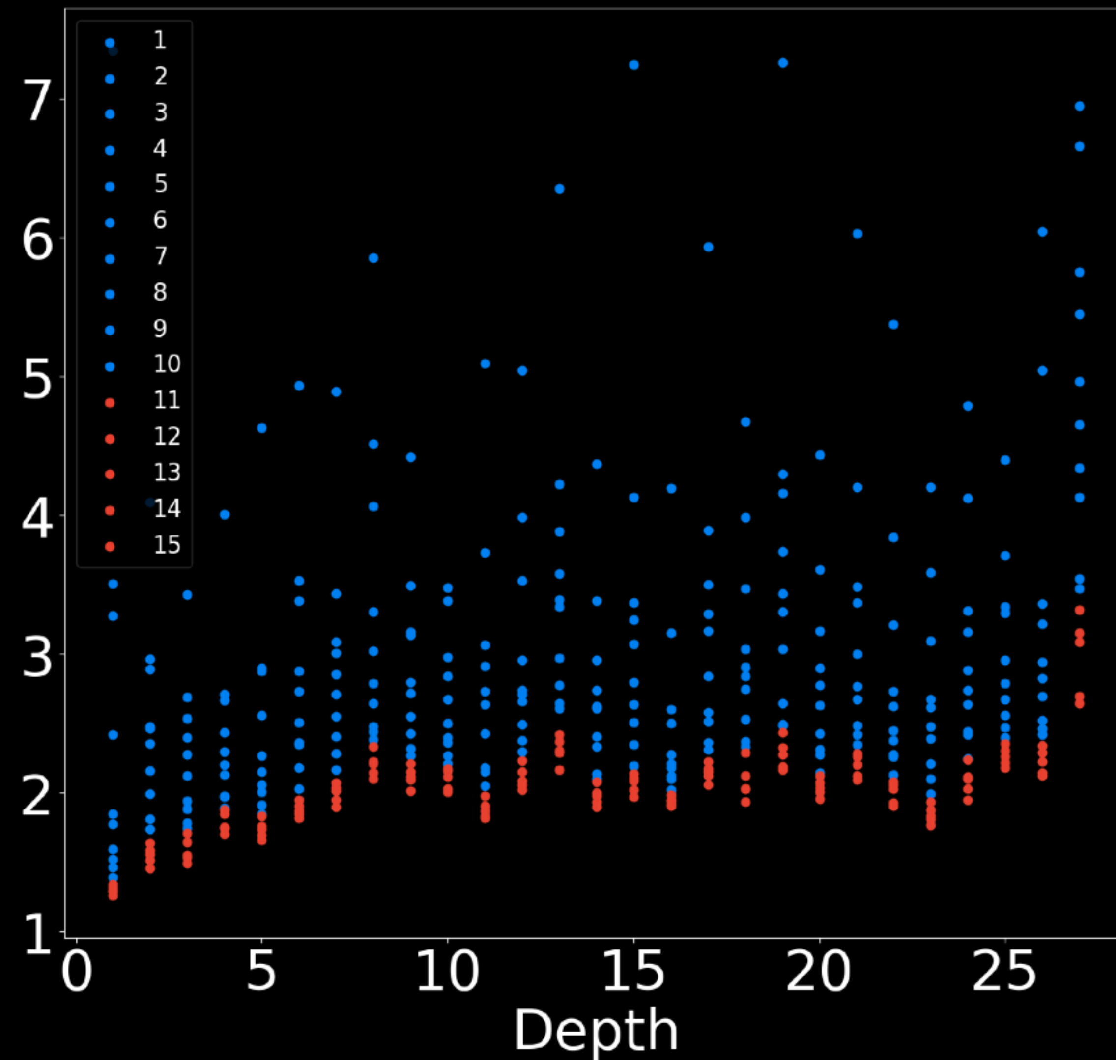
Gemma-7b (Trained)
