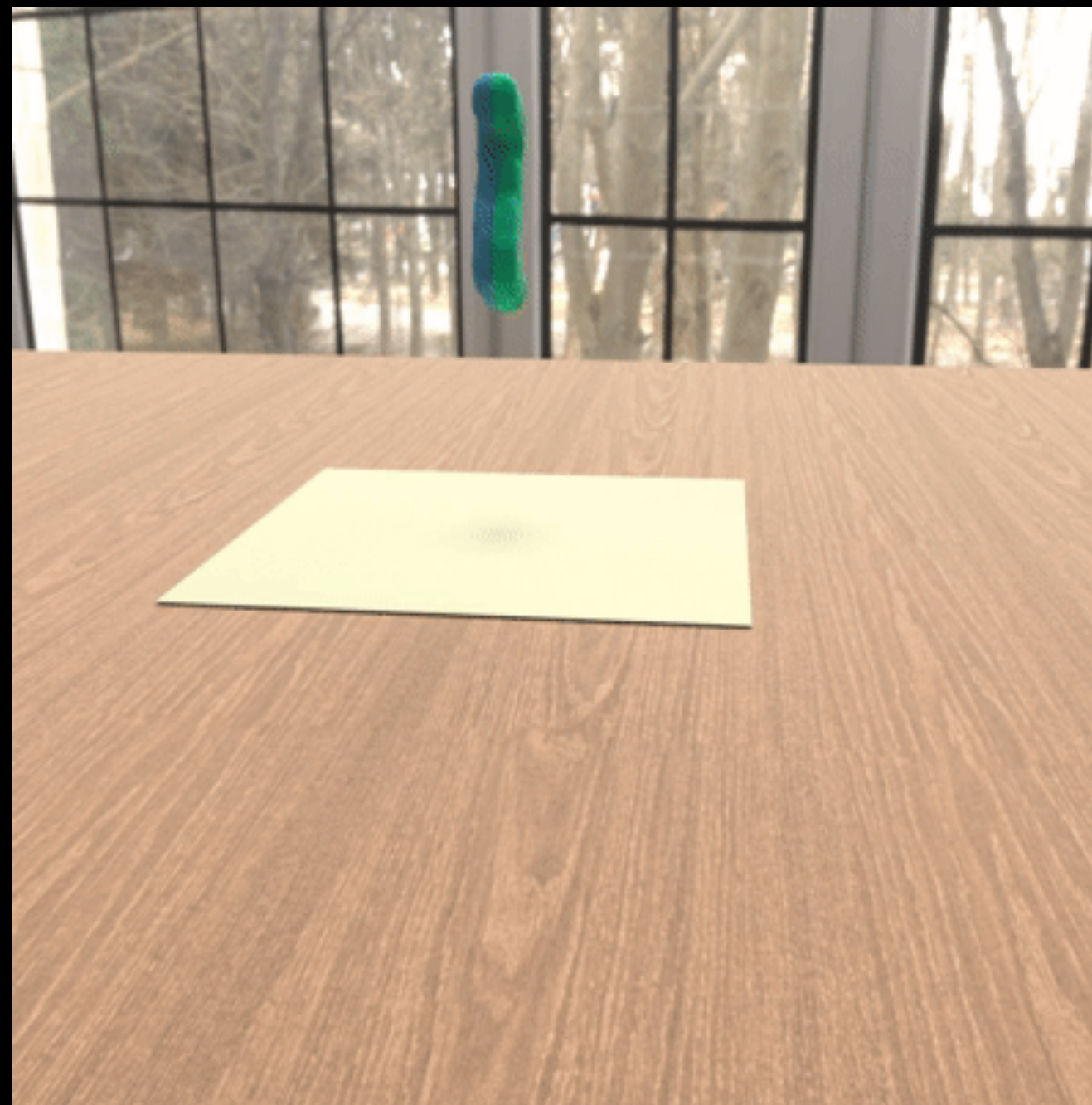
Non-Newtonian
