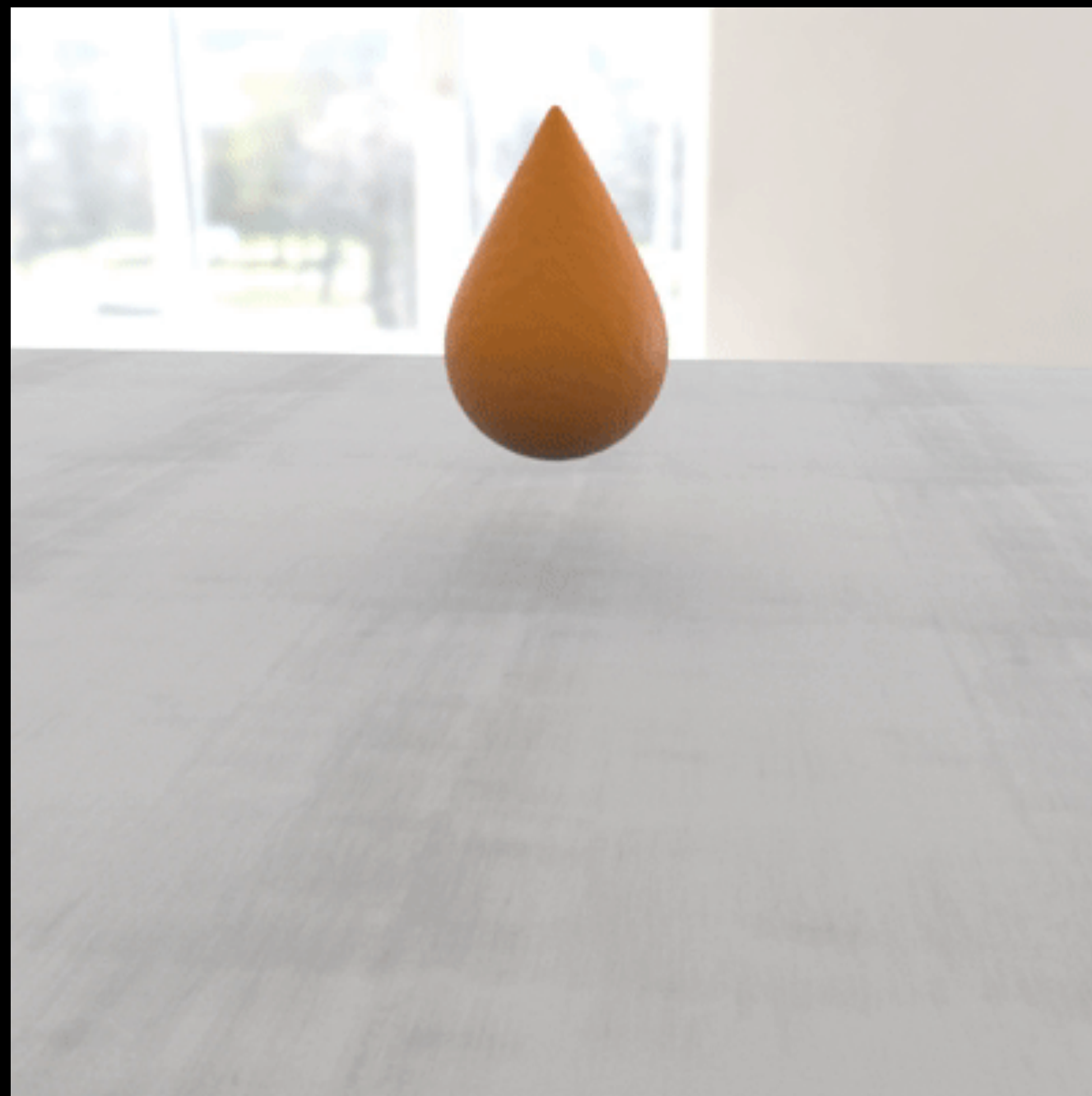
Newtonian
