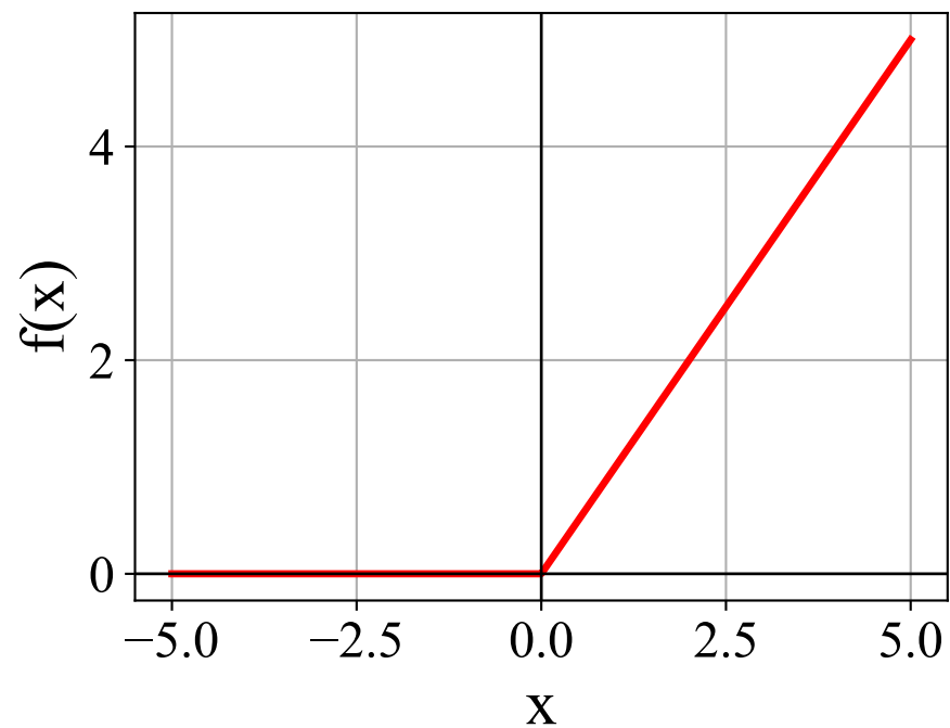
ReLU
