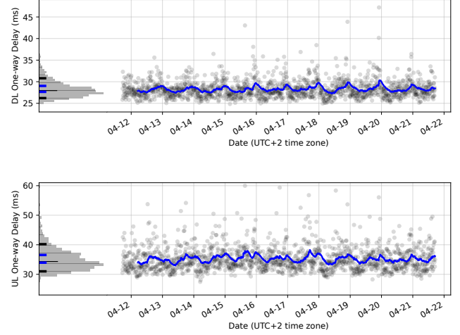
Figure 1: Per-run mean OWD for downlink (DL, upper) and uplink (UL, lower).
