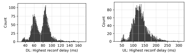
Figure 4: Max OWD within the reconfiguration event
