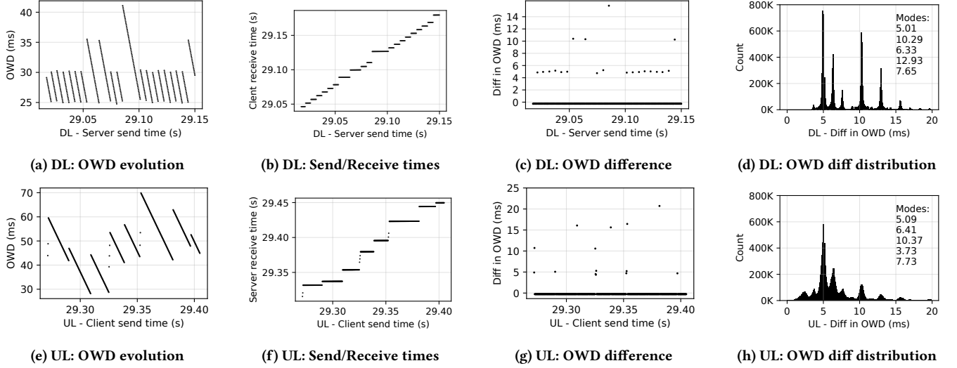
Figure 3: 150 ms zoom-in of run 2025-04-16-09-26-16 (a-c, e-g). Distribution of OWD diff (d, h).
