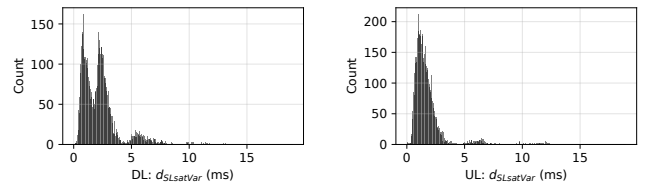
Figure 6: Starlink variable delay component
