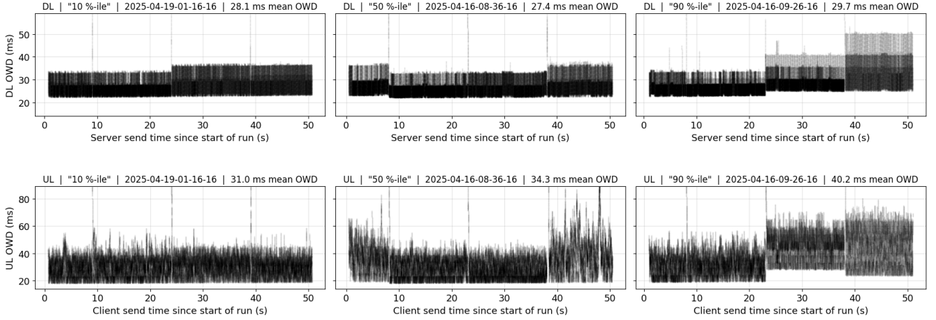
Figure 2: Within-run OWD sample values from 3 selected runs (10, 50, 90th percentile of per-run mean DL/UL OWD). All of the approximately 187K samples per subfigure are plotted.
