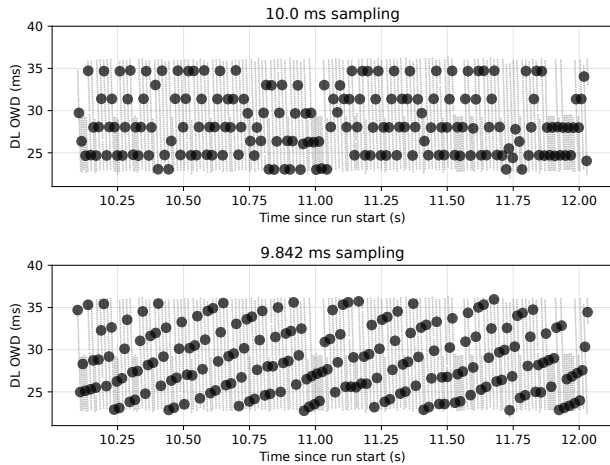
Figure 7: Two examples of aliasing effects for the same data. Simultaneous measurements at both 266 \mu\text{s} intervals (small dots), and at 10 ms and 9.842 ms intervals (large dots)
