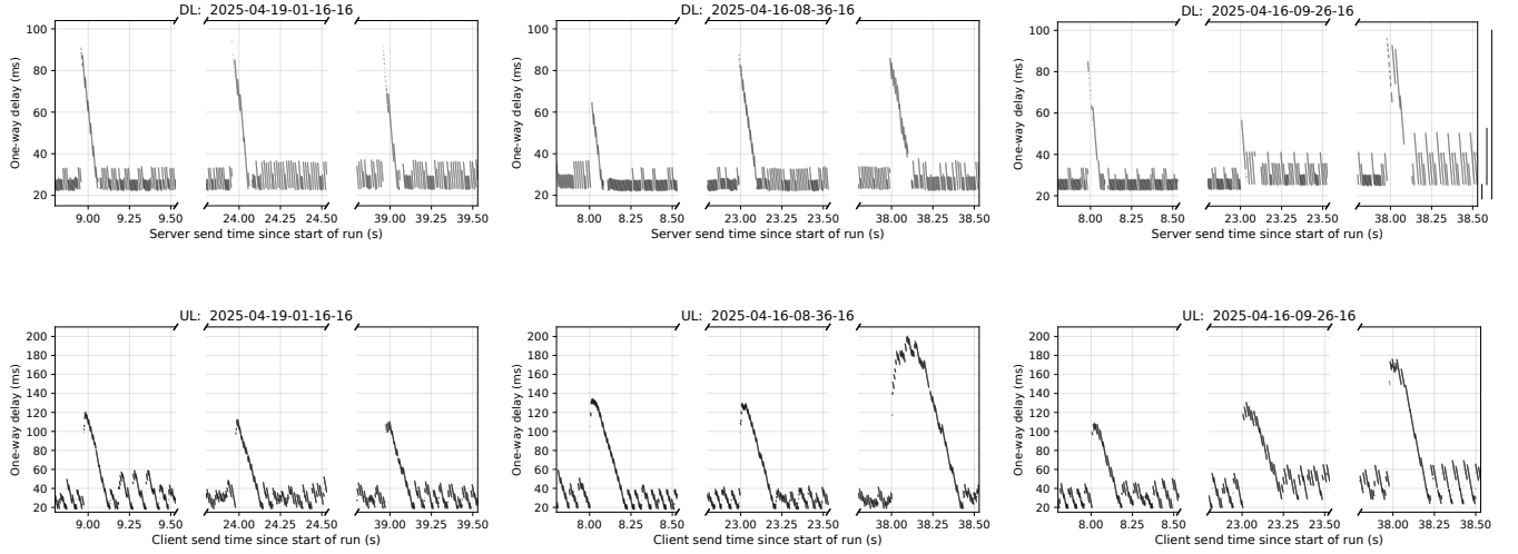
Figure 5: OWD evolution during the reconfiguration events occurring at 15 s intervals
