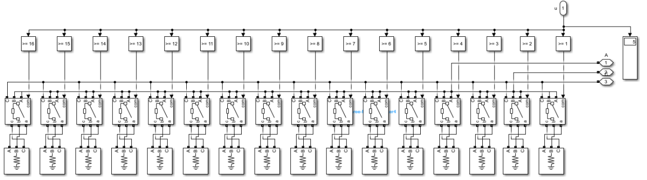
Figure 4: ELC Ballast Load Block in MATLAB/Simulink
