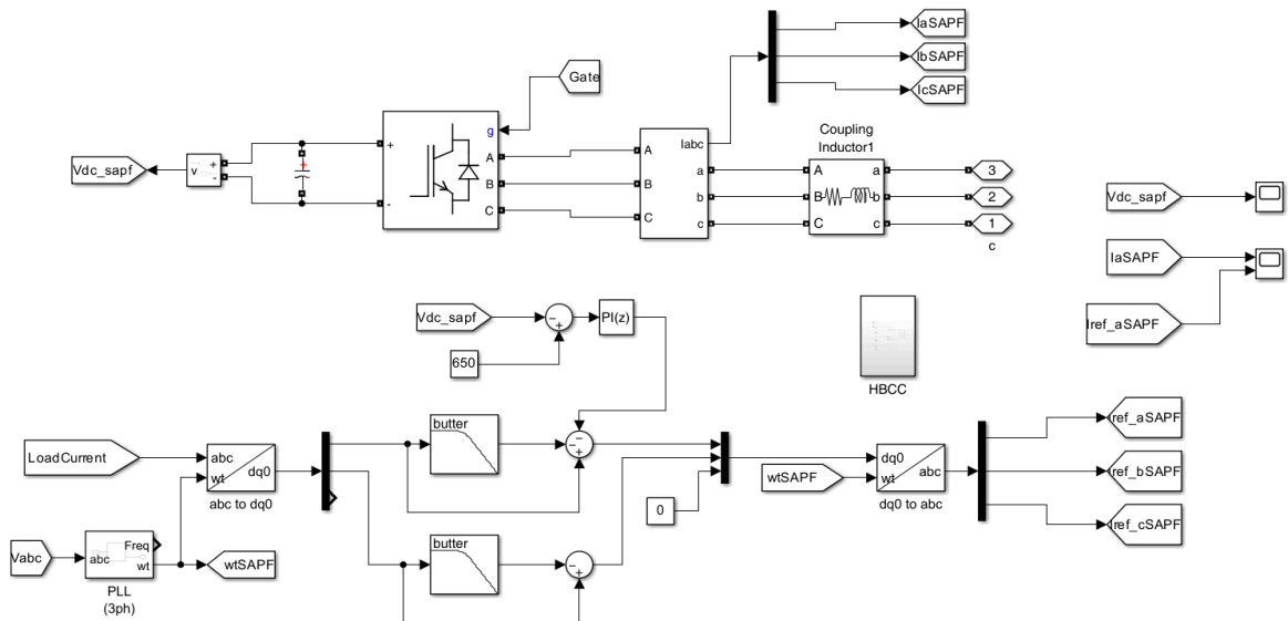
Figure 8: Classical SAPF Block in MATLAB/Simulink
