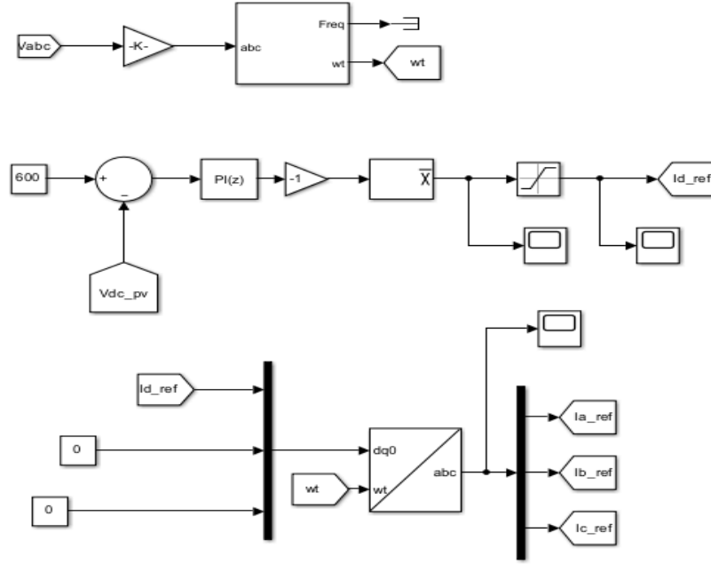
Figure 6: Control Logic Block for Active Power Injection
