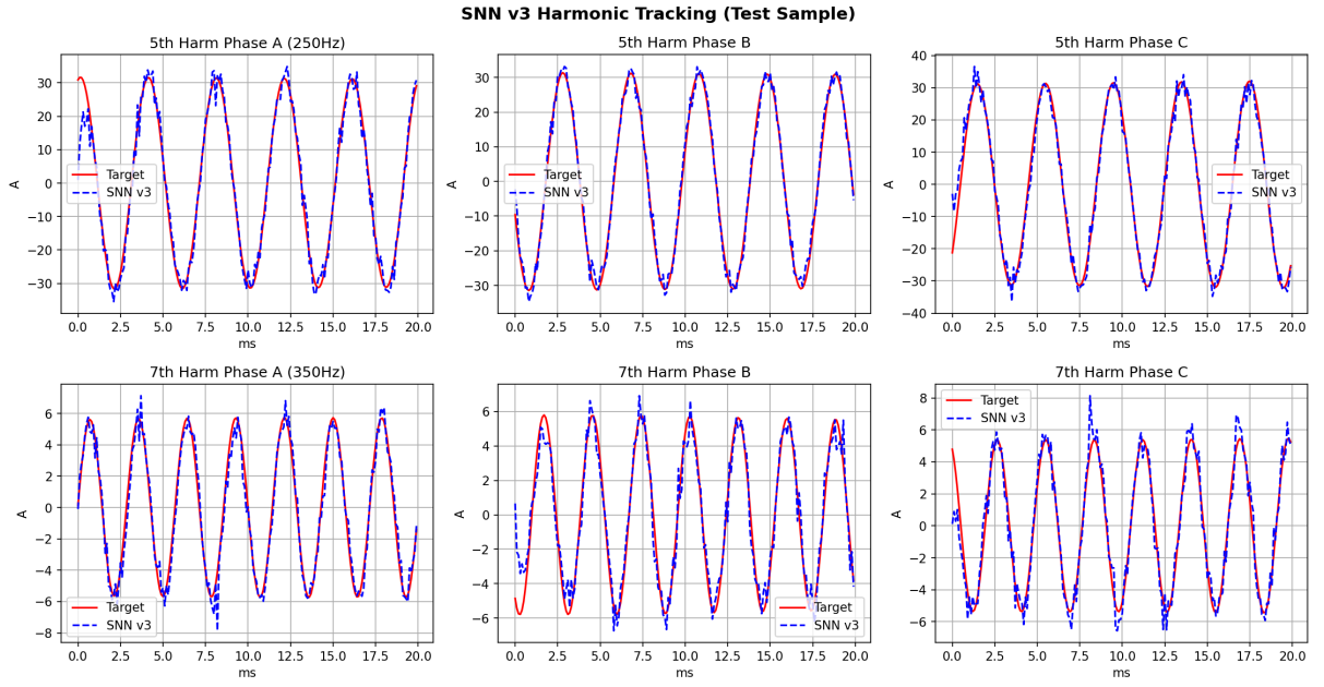
Figure 20: Harmonic Tracking
