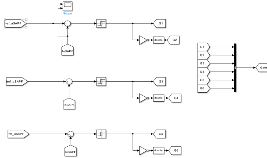
Figure 9: HBCC Block in MATLAB/Simulink
