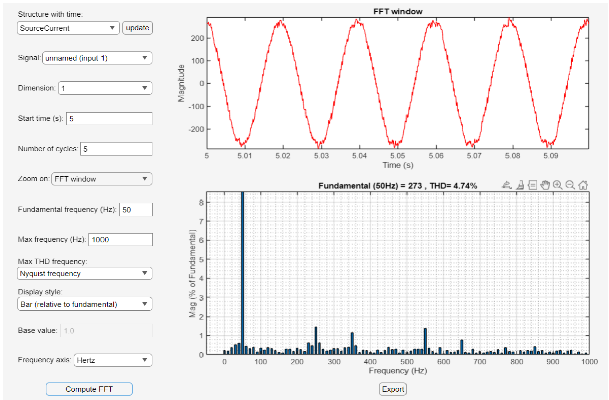
Figure 18: Source Current THD evaluation with SAPF
