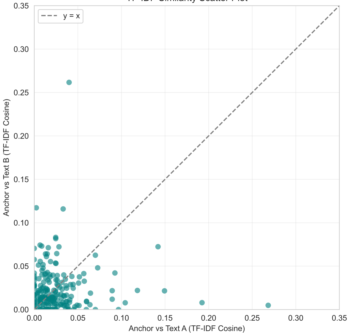
TF-IDF Similarity Scatter Plot
