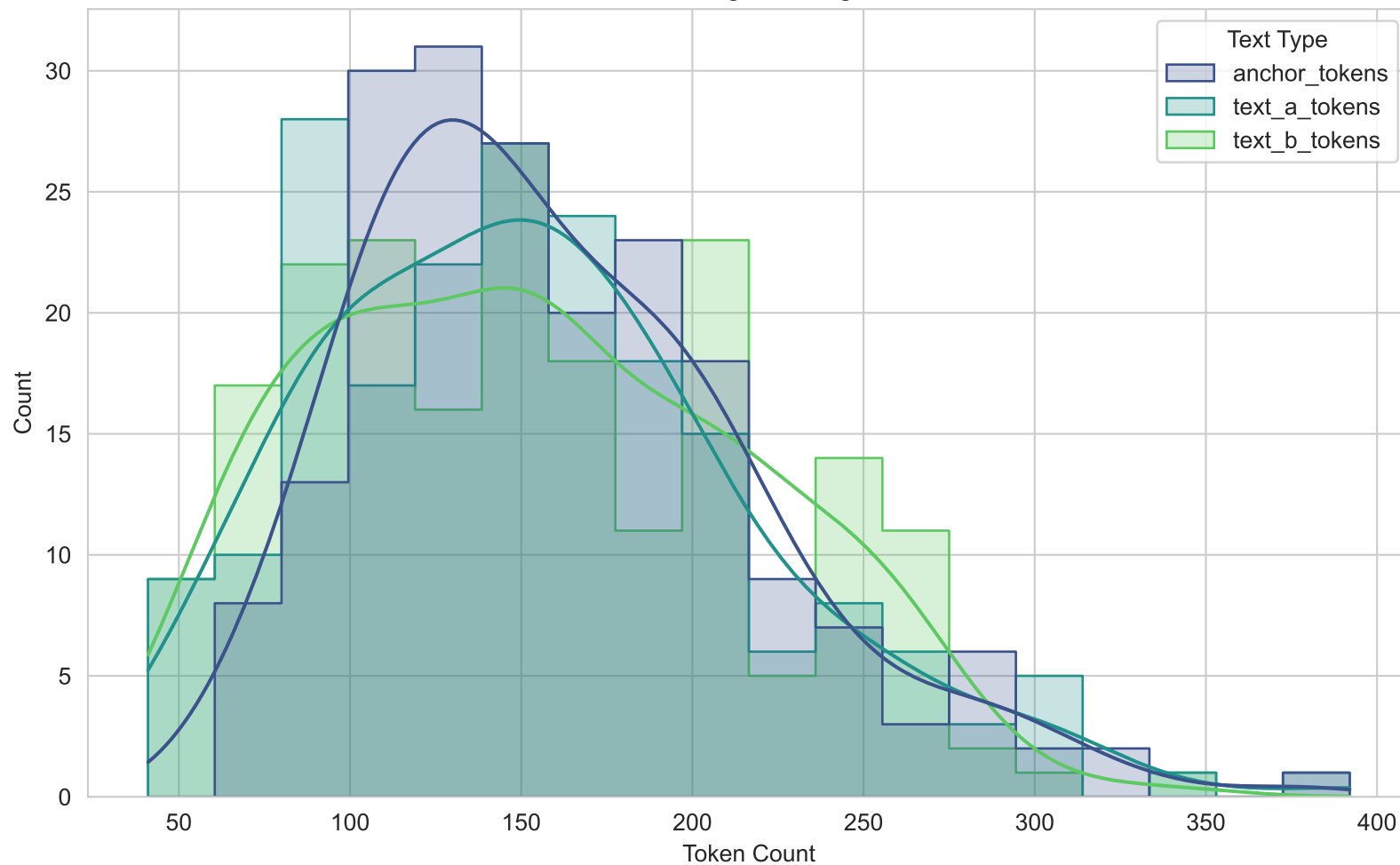
Token Length Histogram
