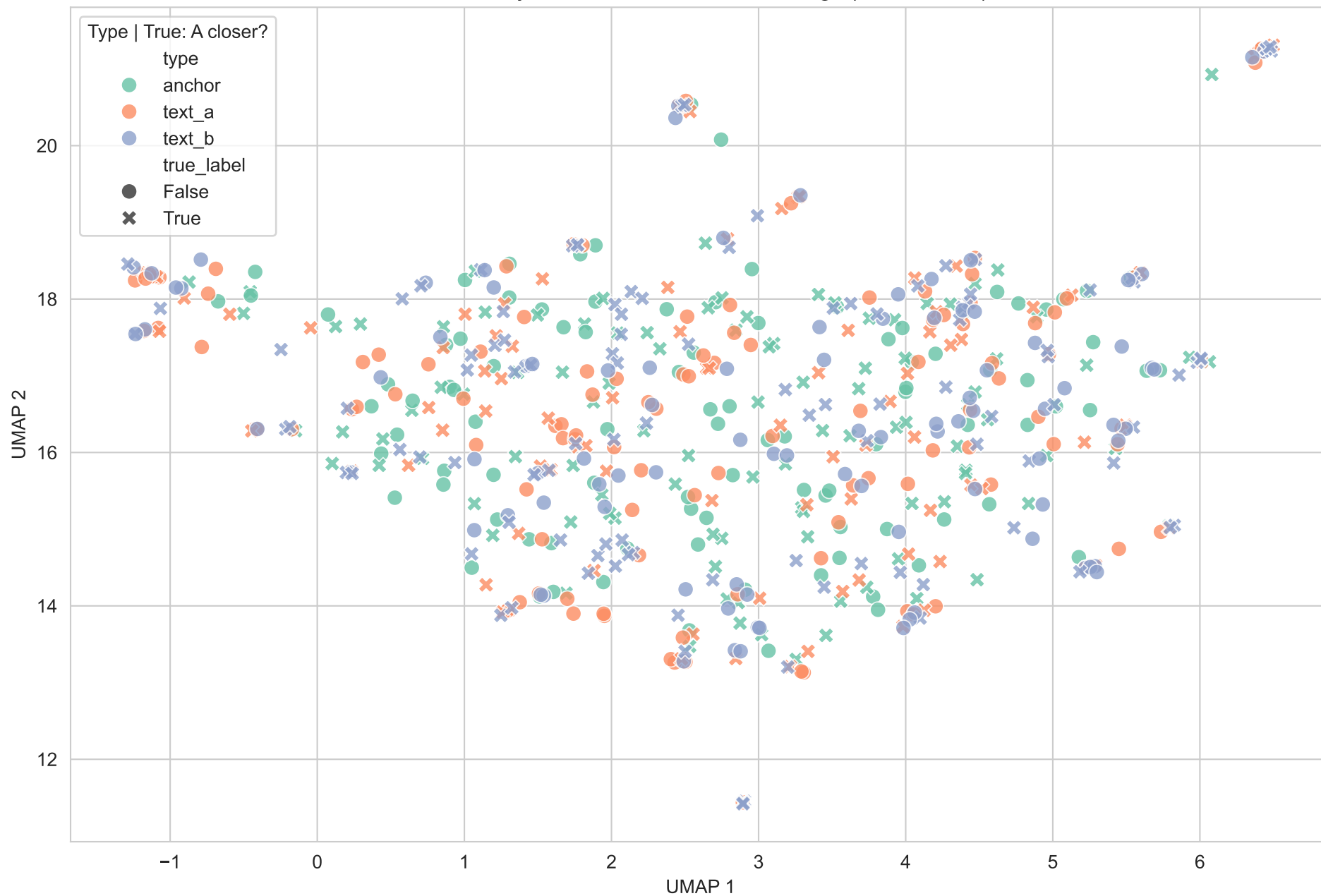
UMAP Projection of Sentence Embeddings (Anchor, A, B)
