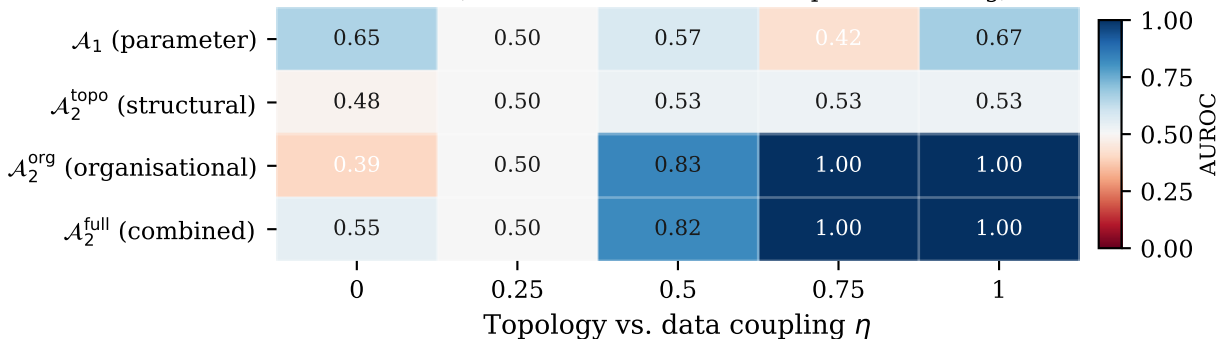
AUROC (red = below chance, blue = perfect ranking)
