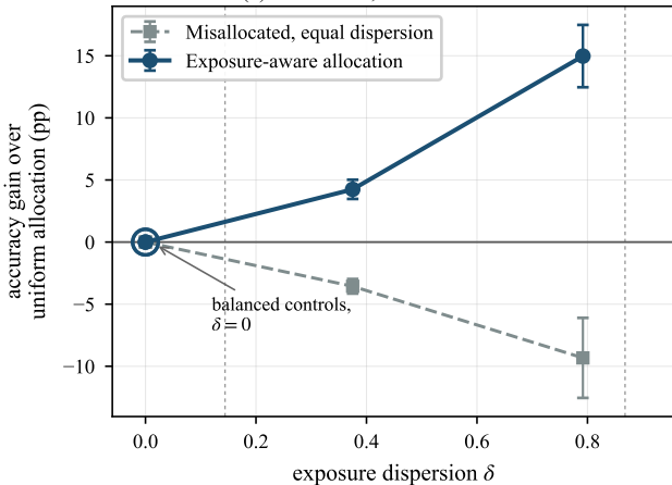
(a) CIFAR-10, frozen ResNet-18
