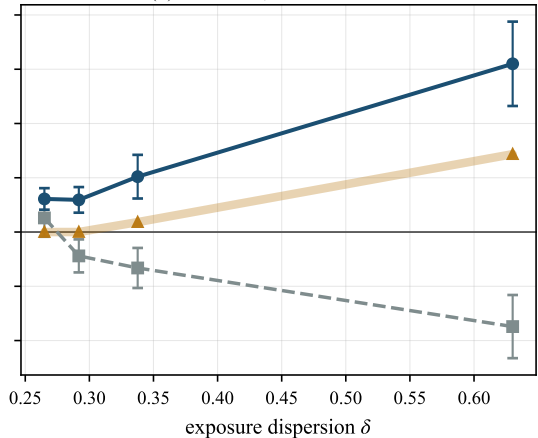
(b) AG News, frozen MiniLM
