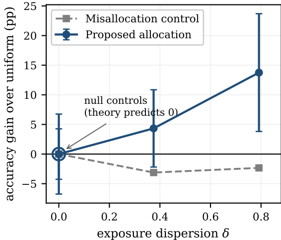
CIFAR-10, frozen ResNet-18
