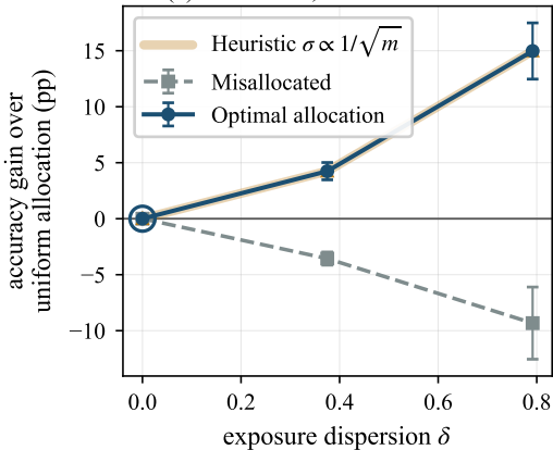
(a) CIFAR-10, frozen ResNet-18
