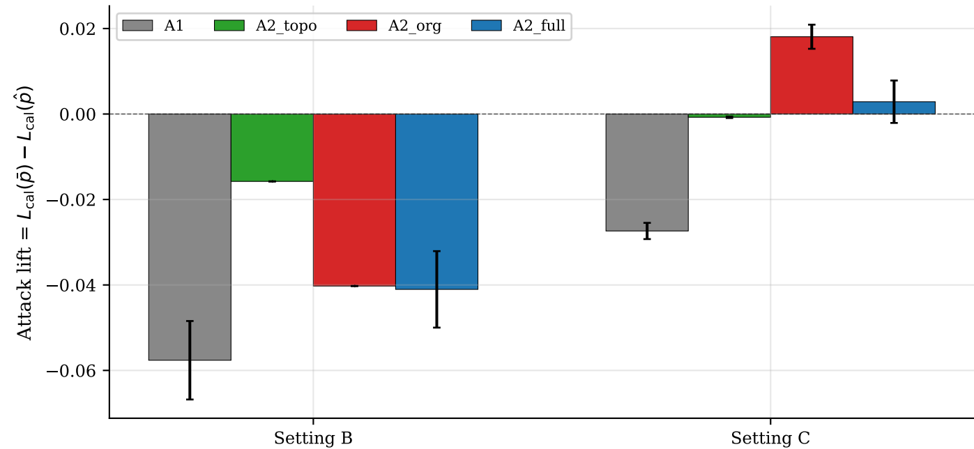
\TADI channel ablation across settings
