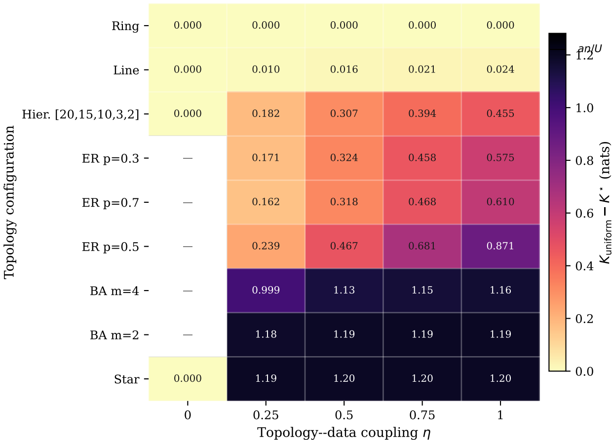
Privacy-bound gap K_{\text{uniform}} - K^* (nats) across topologies
