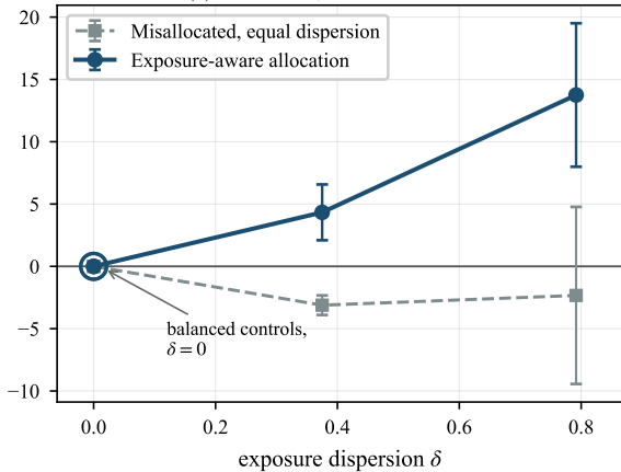
(a) CIFAR-10, frozen ResNet-18
