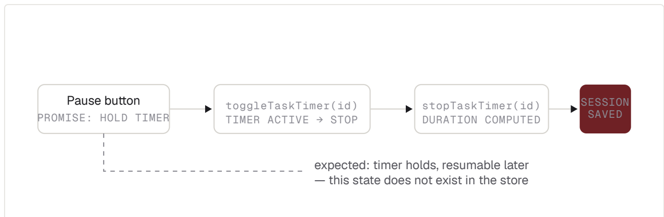
FIG 2 Anatomy of the pause bug. The same call path runs from ActiveTaskTimer , TaskItem 's dialog, and FocusMode .
