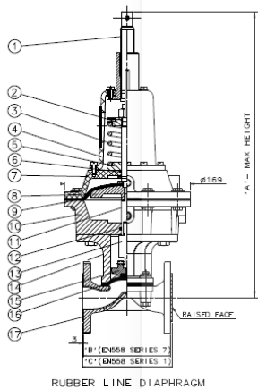
RUBBER LINE DIAPHRAGM
