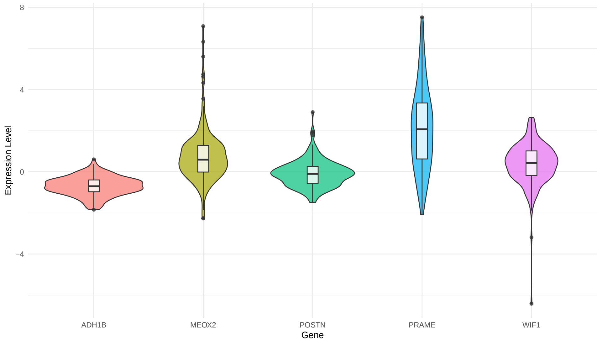
Expression Distribution of Key Sarcoma Biomarkers
