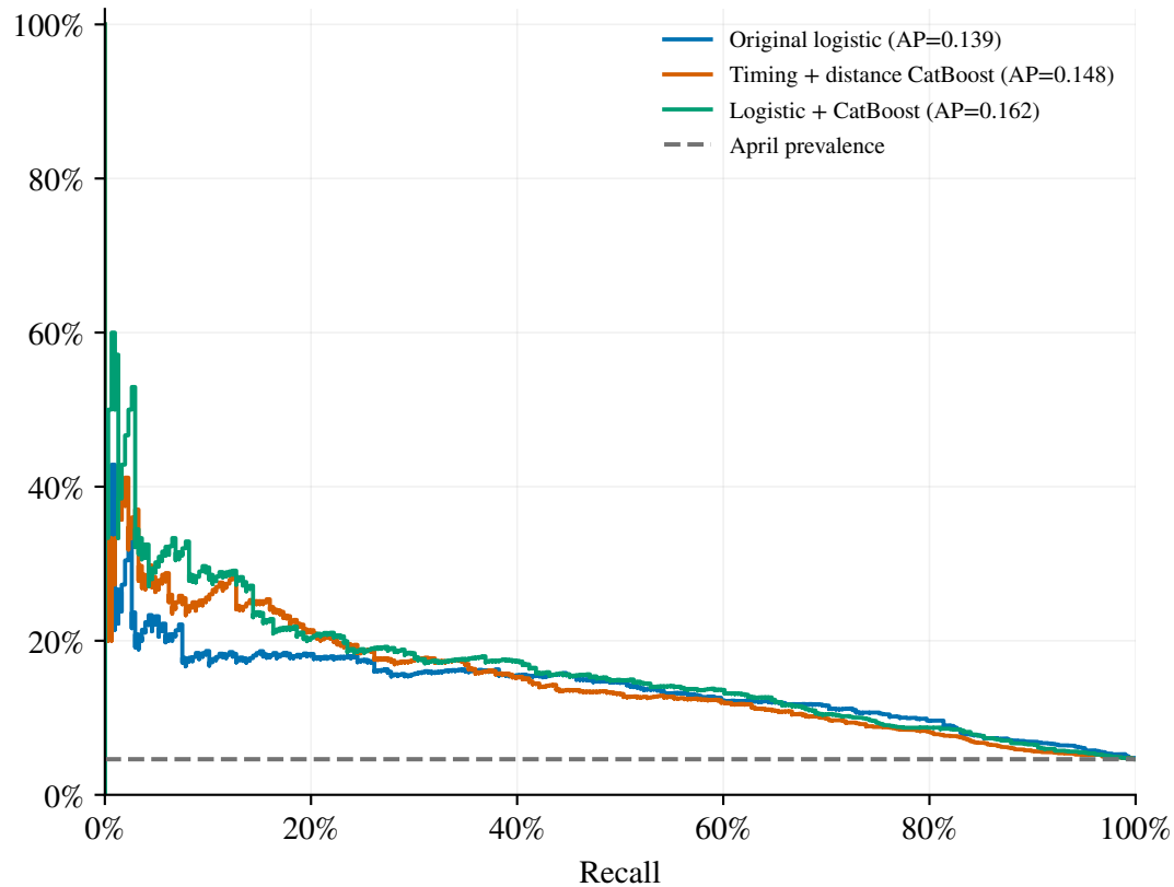
April development precision–recall
