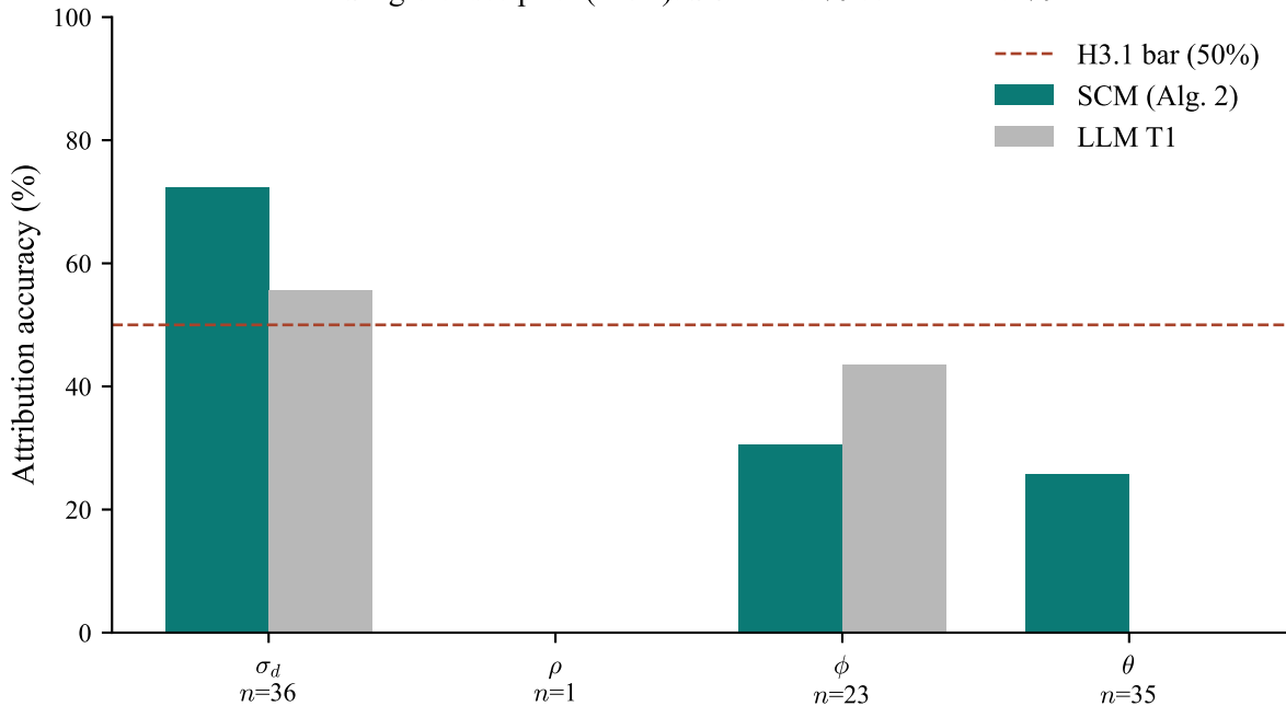
Single-cause pilot (n=95): SCM 44.2% vs LLM 31.6%
