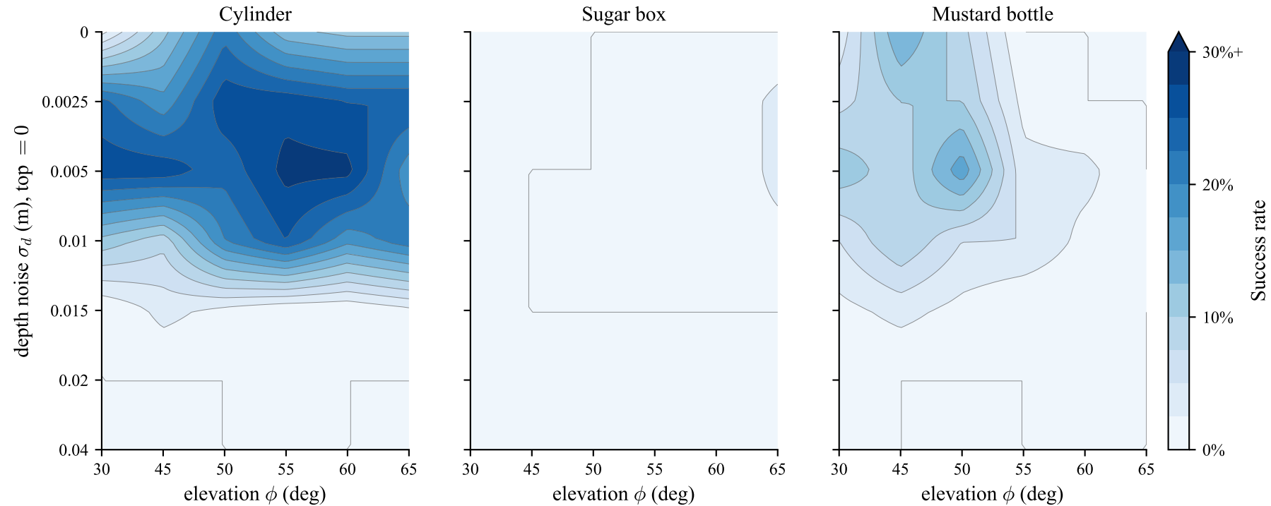
Marginal success (%) by object, depth noise, and elevation (7,560-trial floating-gripper grid, unfiltered top-1, shake)
