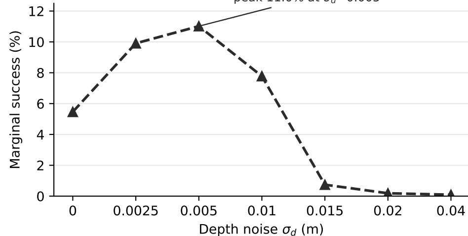
(d) Marginal P(Y=1) against \sigma_d peak 11.0% at \sigma_d=0.005
