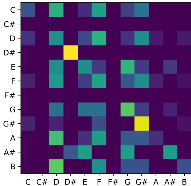
gen-organ-17
