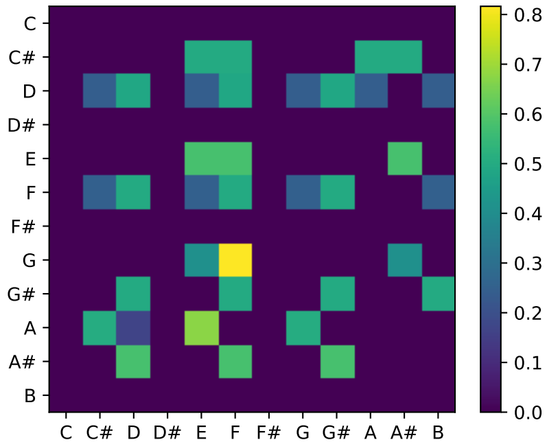
reference-organ-17
