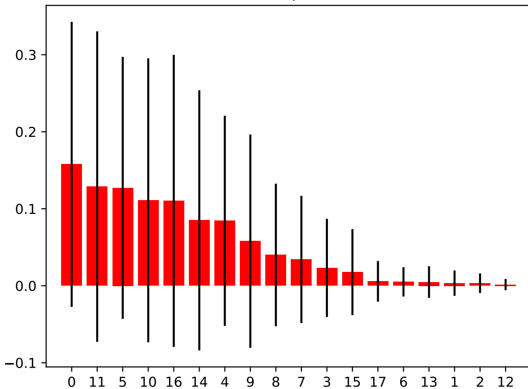
Feature importances
