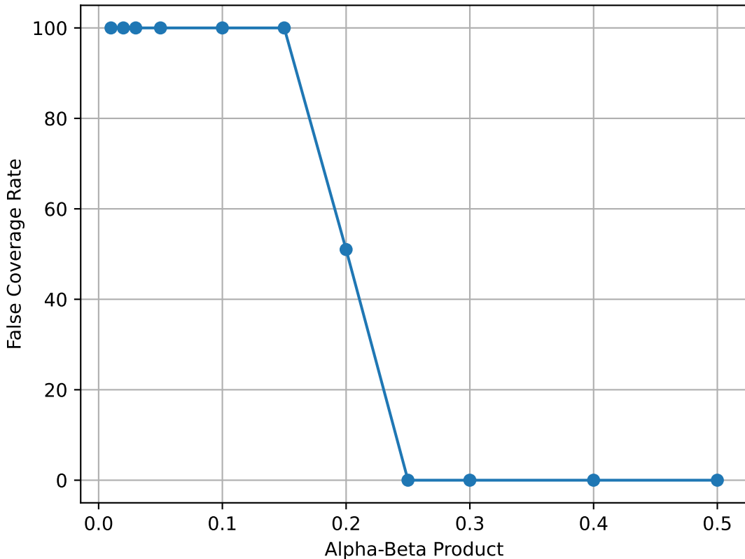
False Coverage Rate vs Alpha-Beta Product
