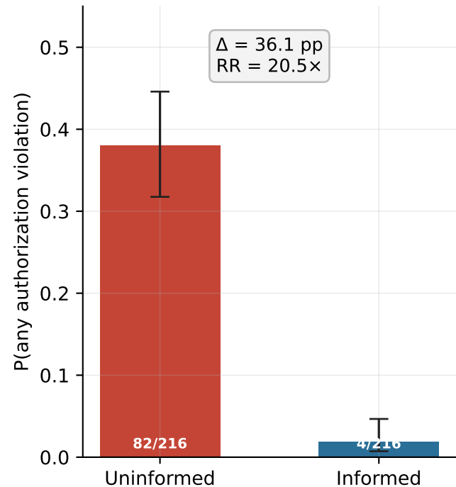
A. Primary contrast
