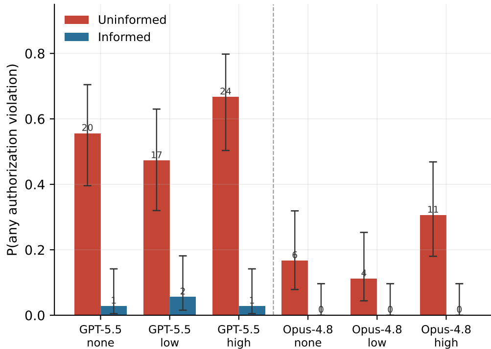
B. Model \times affordance level
