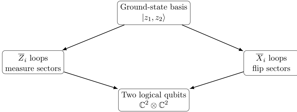
Figure 9.1: Non-contractible anyon string operators act as logical operators on the torus ground-state Hilbert space. The four ground states form two logical qubits.
