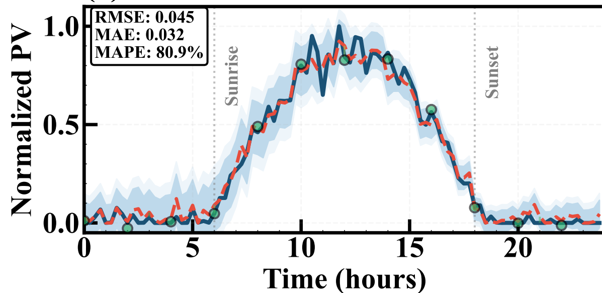
(a) PV Generation Forecast
