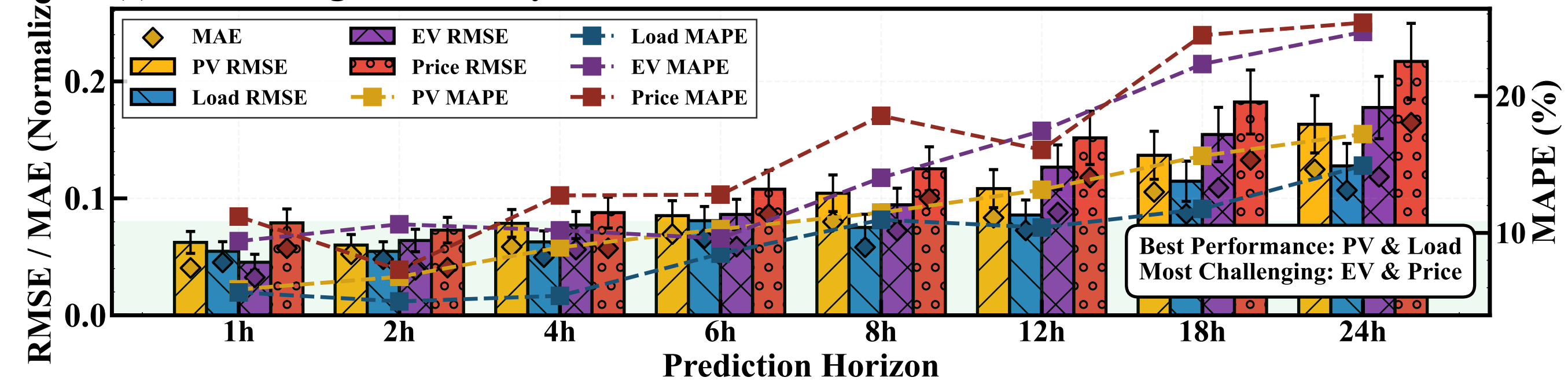
(e) Forecasting Error Analysis - RMSE, MAE, and MAPE Across Horizons
