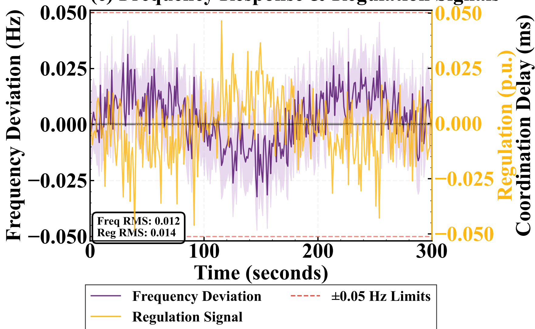
(c) Frequency Response & Regulation Signals
