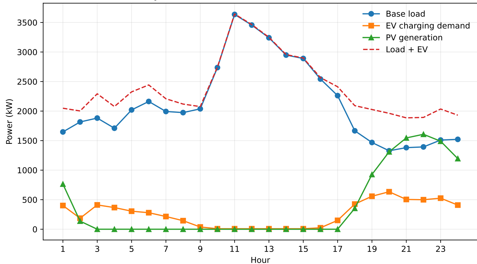
Representative 24-h Demand and PV Profile
